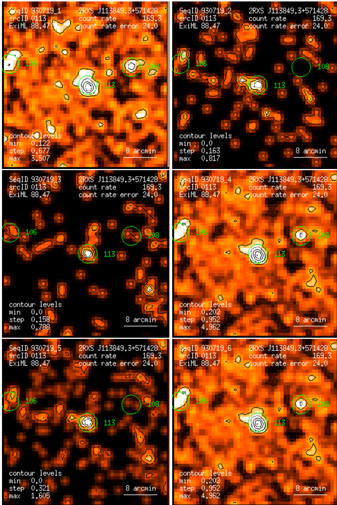
Figure 113: RASS 930719: detection 0113: band rate images, Gaussian filter: (1) PSPC channels 11 – 41, (2) 52 – 90, (3) 91 – 201, (4) 11 – 235, (5) 52 – 201, (6) 11 – 201. Broad band rates in counts/ks. Band rate contour levels in counts/ks/arcmin 2 .
