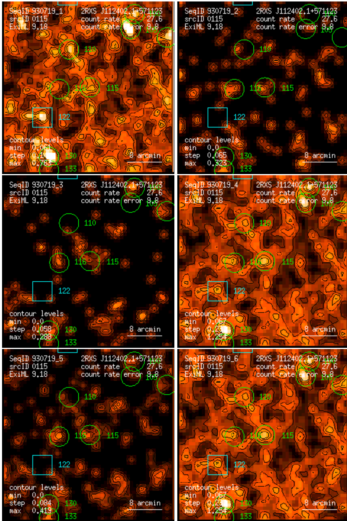
Figure 115: RASS 930719: detection 0115: band rate images, Gaussian filter: (1) PSPC channels 11 – 41, (2) 52 – 90, (3) 91 – 201, (4) 11 – 235, (5) 52 – 201, (6) 11 – 201. Broad band rates in counts/ks. Band rate contour levels in counts/ks/arcmin 2 .
