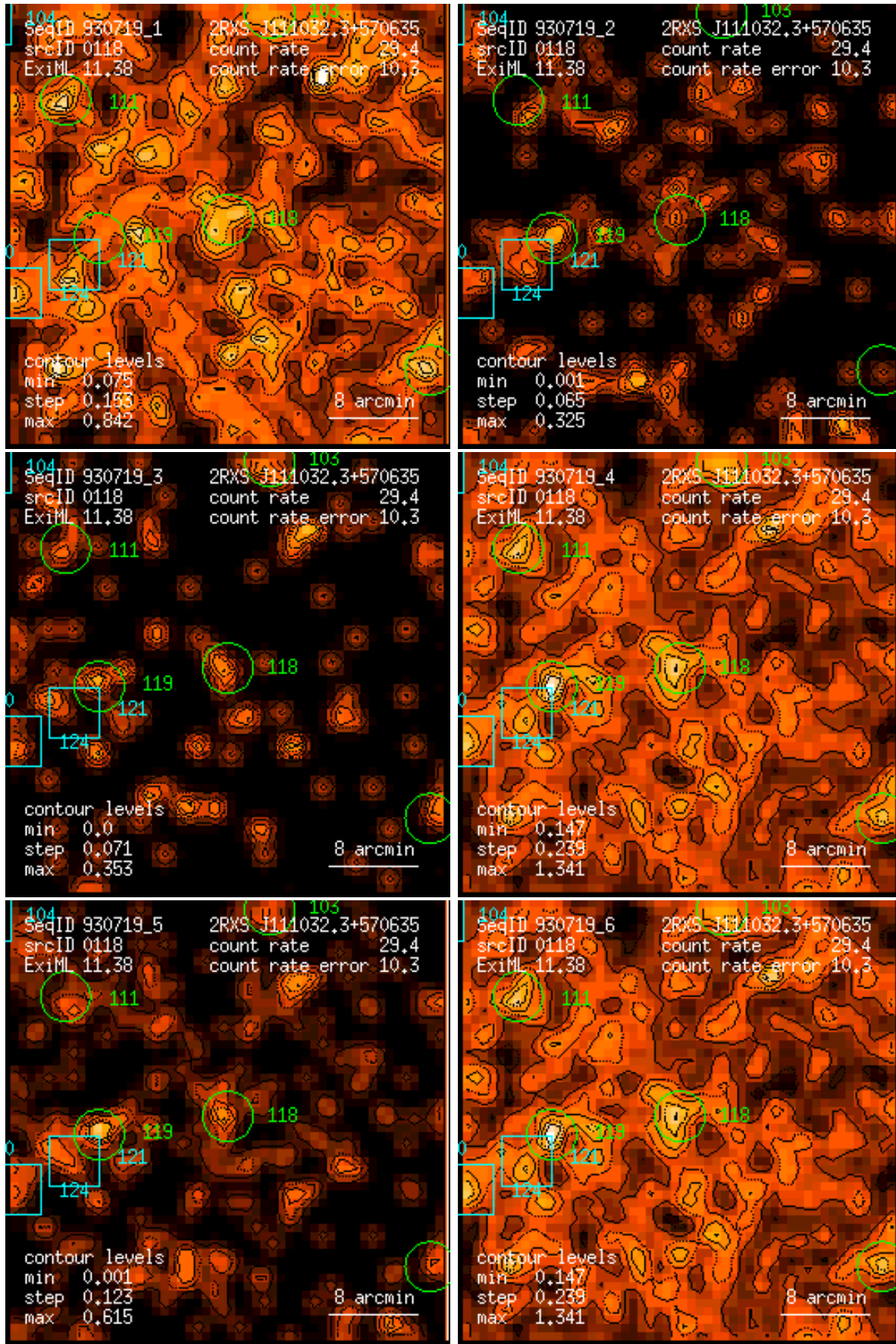
Figure 118: RASS 930719: detection 0118: band rate images, Gaussian filter: (1) PSPC channels 11 – 41, (2) 52 – 90, (3) 91 – 201, (4) 11 – 235, (5) 52 – 201, (6) 11 – 201. Broad band rates in counts/ks. Band rate contour levels in counts/ks/arcmin 2 .
