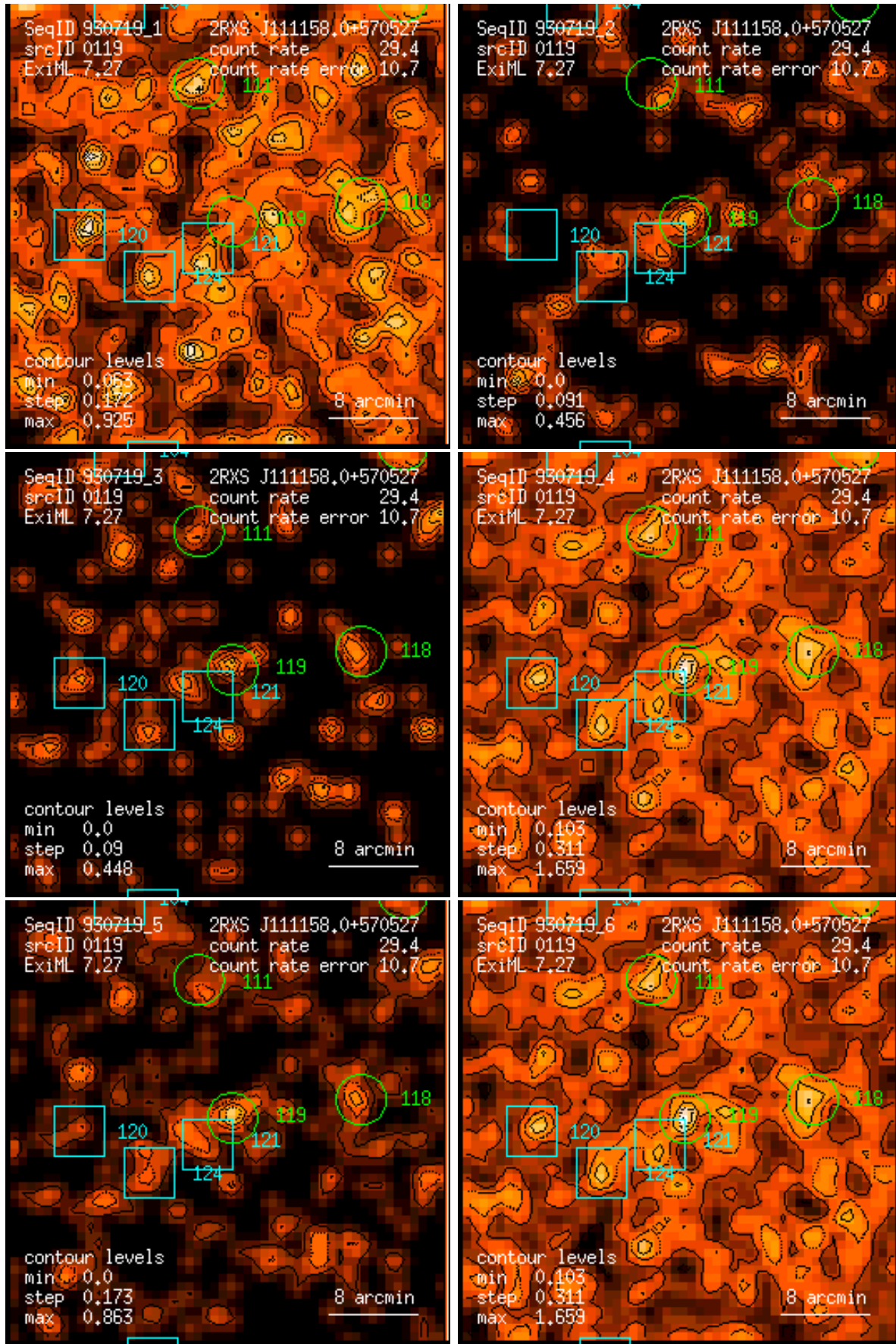
Figure 119: RASS 930719: detection 0119: band rate images, Gaussian filter: (1) PSPC channels 11 – 41, (2) 52 – 90, (3) 91 – 201, (4) 11 – 235, (5) 52 – 201, (6) 11 – 201. Broad band rates in counts/ks. Band rate contour levels in counts/ks/arcmin 2 .
