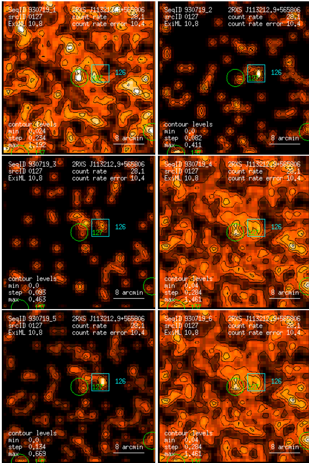
Figure 127: RASS 930719: detection 0127: band rate images, Gaussian filter: (1) PSPC channels 11 – 41, (2) 52 – 90, (3) 91 – 201, (4) 11 – 235, (5) 52 – 201, (6) 11 – 201. Broad band rates in counts/ks. Band rate contour levels in counts/ks/arcmin 2 .
