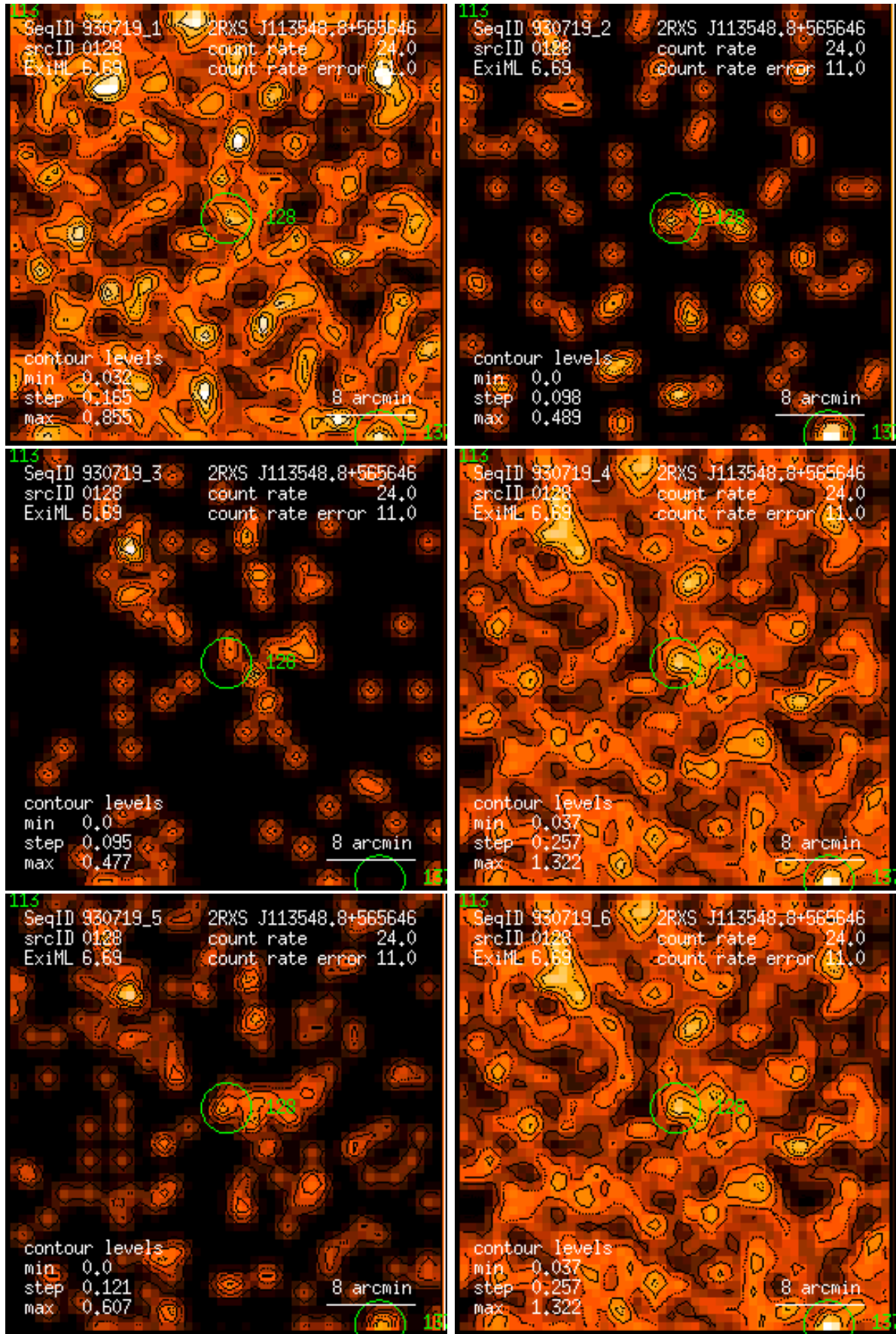
Figure 128: RASS 930719: detection 0128: band rate images, Gaussian filter: (1) PSPPC channels 11 – 41, (2) 52 – 90, (3) 91 – 201, (4) 11 – 235, (5) 52 – 201, (6) 11 – 201. Broad band rates in counts/ks. Band rate contour levels in counts/ks/arcmin 2 .
