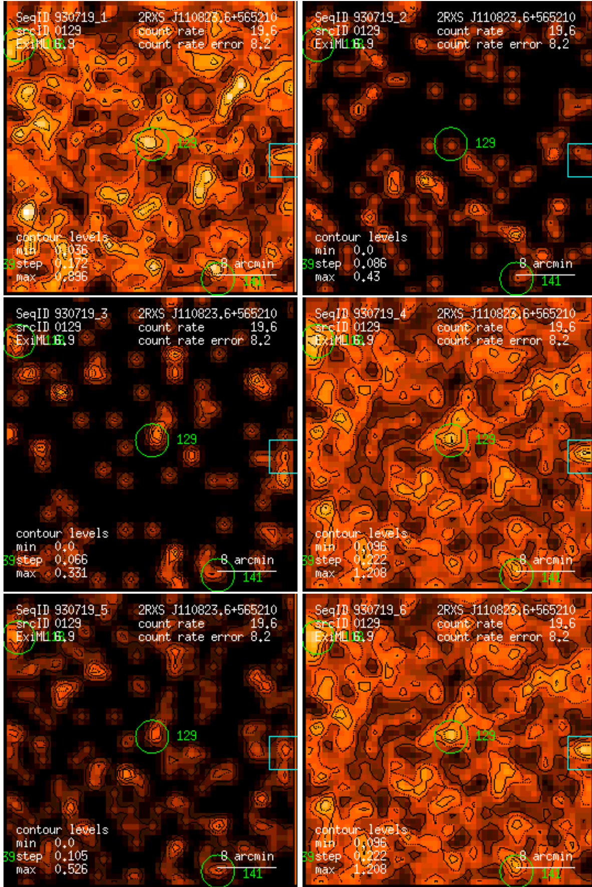
Figure 129: RASS 930719: detection 0129: band rate images, Gaussian filter: (1) PSPC channels 11 – 41, (2) 52 – 90, (3) 91 – 201, (4) 11 – 235, (5) 52 – 201, (6) 11 – 201. Broad band rates in counts/ks. Band rate contour levels in counts/ks/arcmin 2 .
