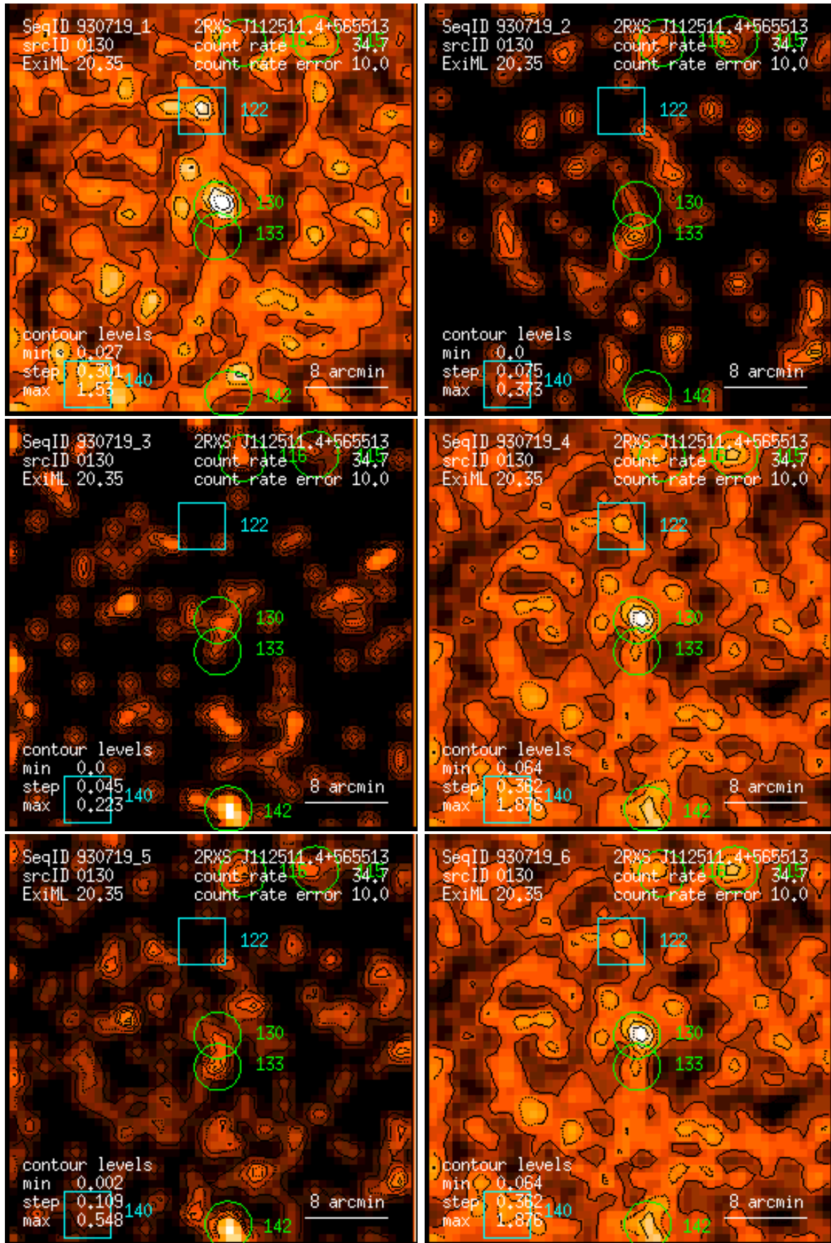
Figure 130: RASS 930719: detection 0130: band rate images, Gaussian filter: (1) PSPC channels 11 – 41, (2) 52 – 90, (3) 91 – 201, (4) 11 – 235, (5) 52 – 201, (6) 11 – 201. Broad band rates in counts/ks. Band rate contour levels in counts/ks/arcmin 2 .
