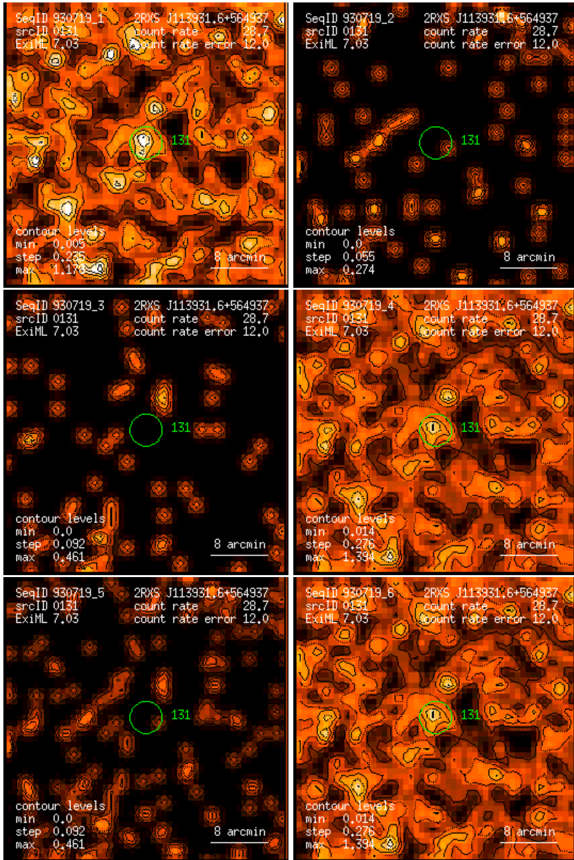
Figure 131: RASS 930719: detection 0131: band rate images, Gaussian filter: (1) PSPC channels 11 – 41, (2) 52 – 90, (3) 91 – 201, (4) 11 – 235, (5) 52 – 201, (6) 11 – 201. Broad band rates in counts/ks. Band rate contour levels in counts/ks/arcmin 2 .
