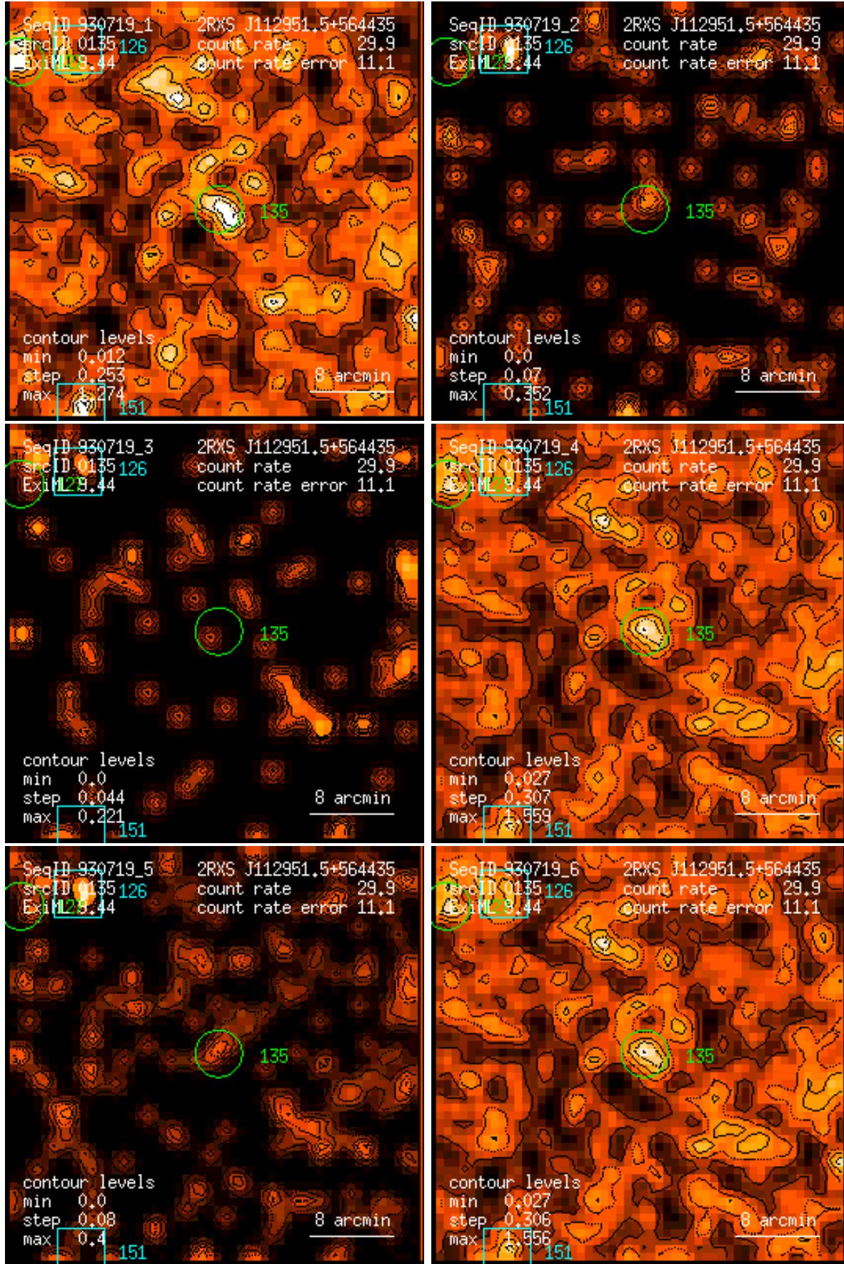
Figure 135: RASS 930719: detection 0135: band rate images, Gaussian filter: (1) PSPC channels 11 – 41, (2) 52 – 90, (3) 91 – 201, (4) 11 – 235, (5) 52 – 201, (6) 11 – 201. Broad band rates in counts/ks. Band rate contour levels in counts/ks/arcmin 2 .
