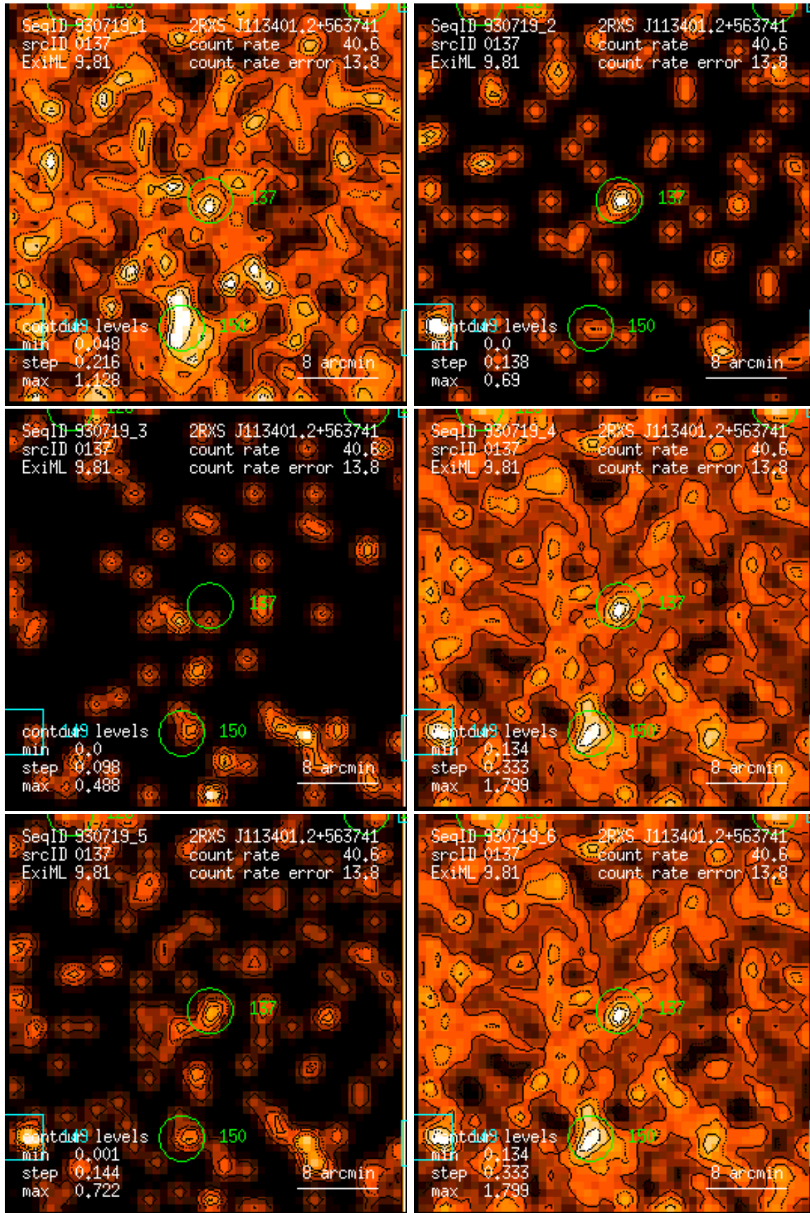
Figure 137: RASS 930719: detection 0137: band rate images, Gaussian filter: (1) PSPC channels 11 – 41, (2) 52 – 90, (3) 91 – 201, (4) 11 – 235, (5) 52 – 201, (6) 11 – 201. Broad band rates in counts/ks. Band rate contour levels in counts/ks/arcmin 2 .
