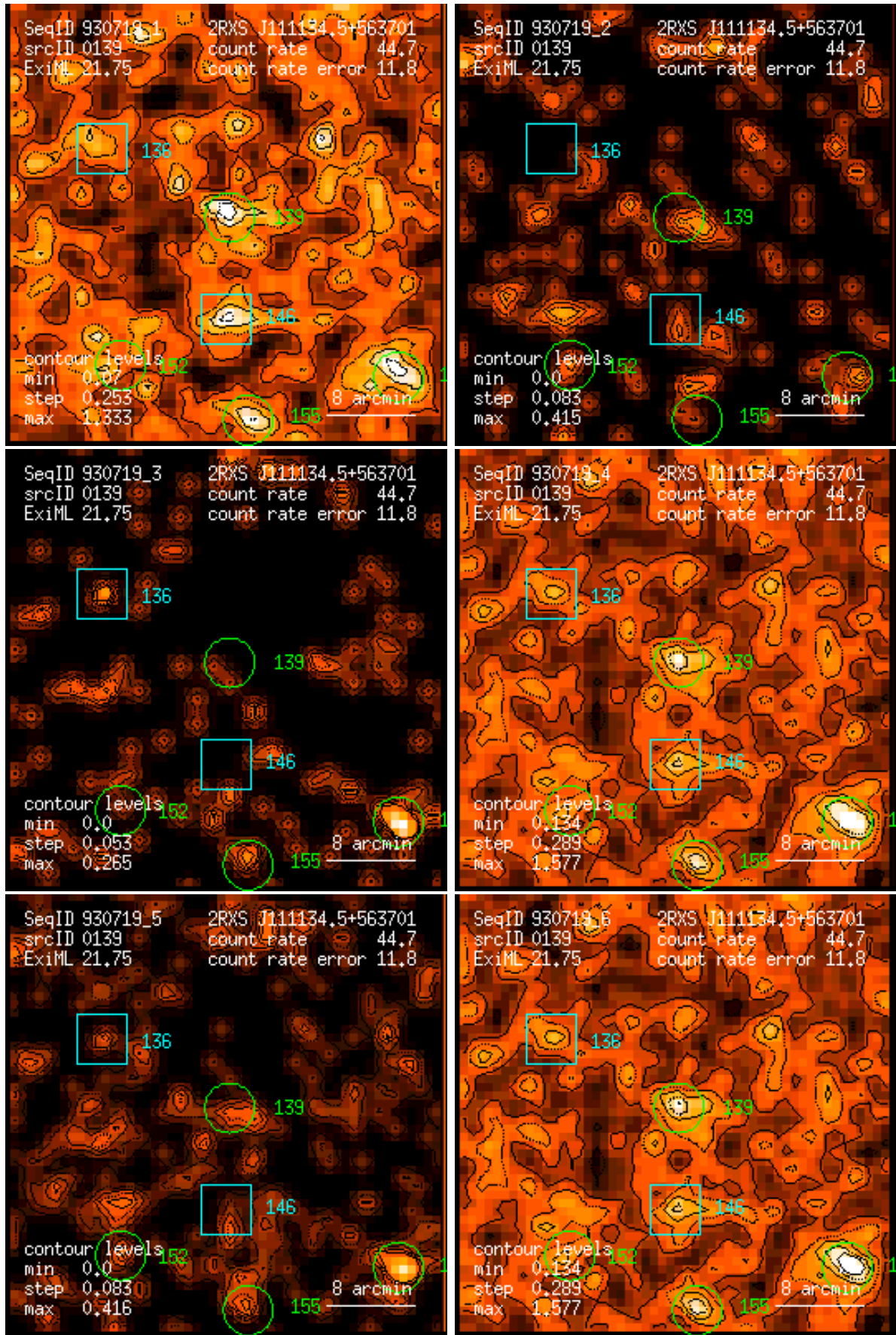
Figure 139: RASS 930719: detection 0139: band rate images, Gaussian filter: (1) PSPC channels 11 – 41, (2) 52 – 90, (3) 91 – 201, (4) 11 – 235, (5) 52 – 201, (6) 11 – 201. Broad band rates in counts/ks. Band rate contour levels in counts/ks/arcmin 2 .
