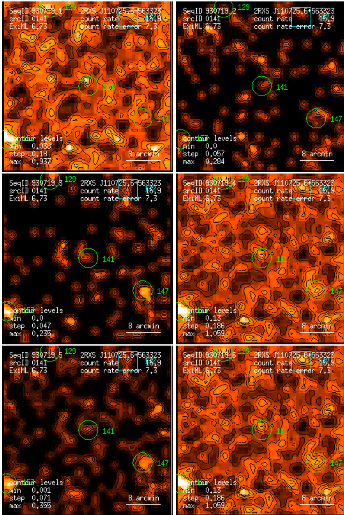
Figure 141: RASS 930719: detection 0141: band rate images, Gaussian filter: (1) PSPC channels 11 – 41, (2) 52 – 90, (3) 91 – 201, (4) 11 – 235, (5) 52 – 201, (6) 11 – 201. Broad band rates in counts/ks. Band rate contour levels in counts/ks/arcmin 2 .
