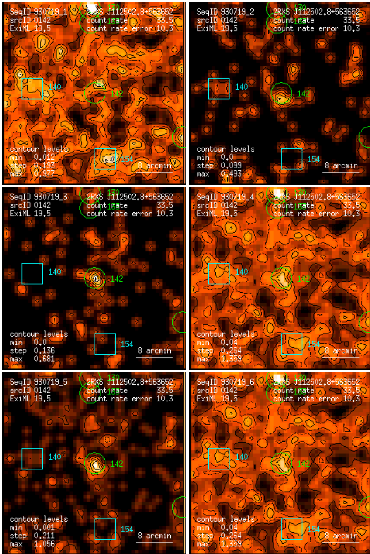
Figure 142: RASS 930719: detection 0142: band rate images, Gaussian filter: (1) PSPC channels 11 – 41, (2) 52 – 90, (3) 91 – 201, (4) 11 – 235, (5) 52 – 201, (6) 11 – 201. Broad band rates in counts/ks. Band rate contour levels in counts/ks/arcmin 2 .
