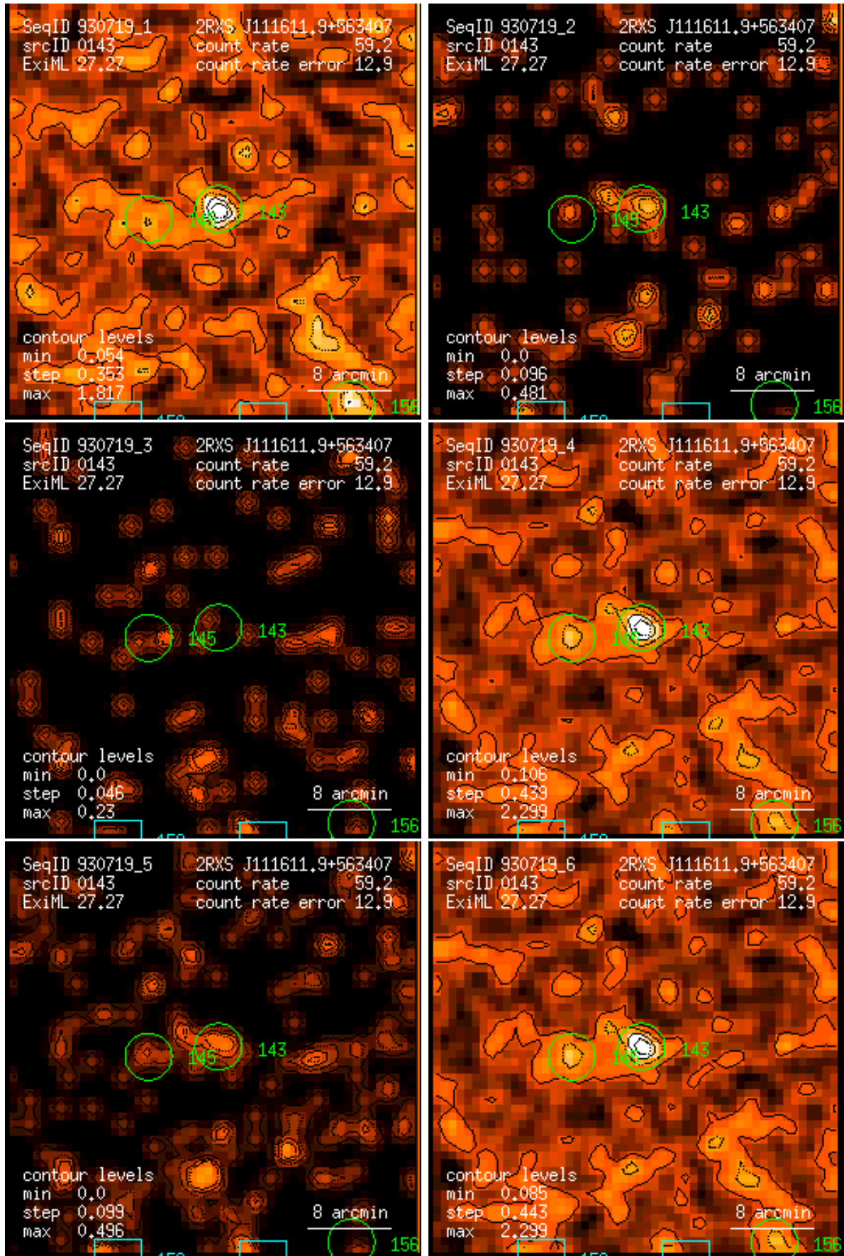
Figure 143: RASS 930719: detection 0143: band rate images, Gaussian filter: (1) PSPC channels 11 – 41, (2) 52 – 90, (3) 91 – 201, (4) 11 – 235, (5) 52 – 201, (6) 11 – 201. Broad band rates in counts/ks. Band rate contour levels in counts/ks/arcmin 2 .
