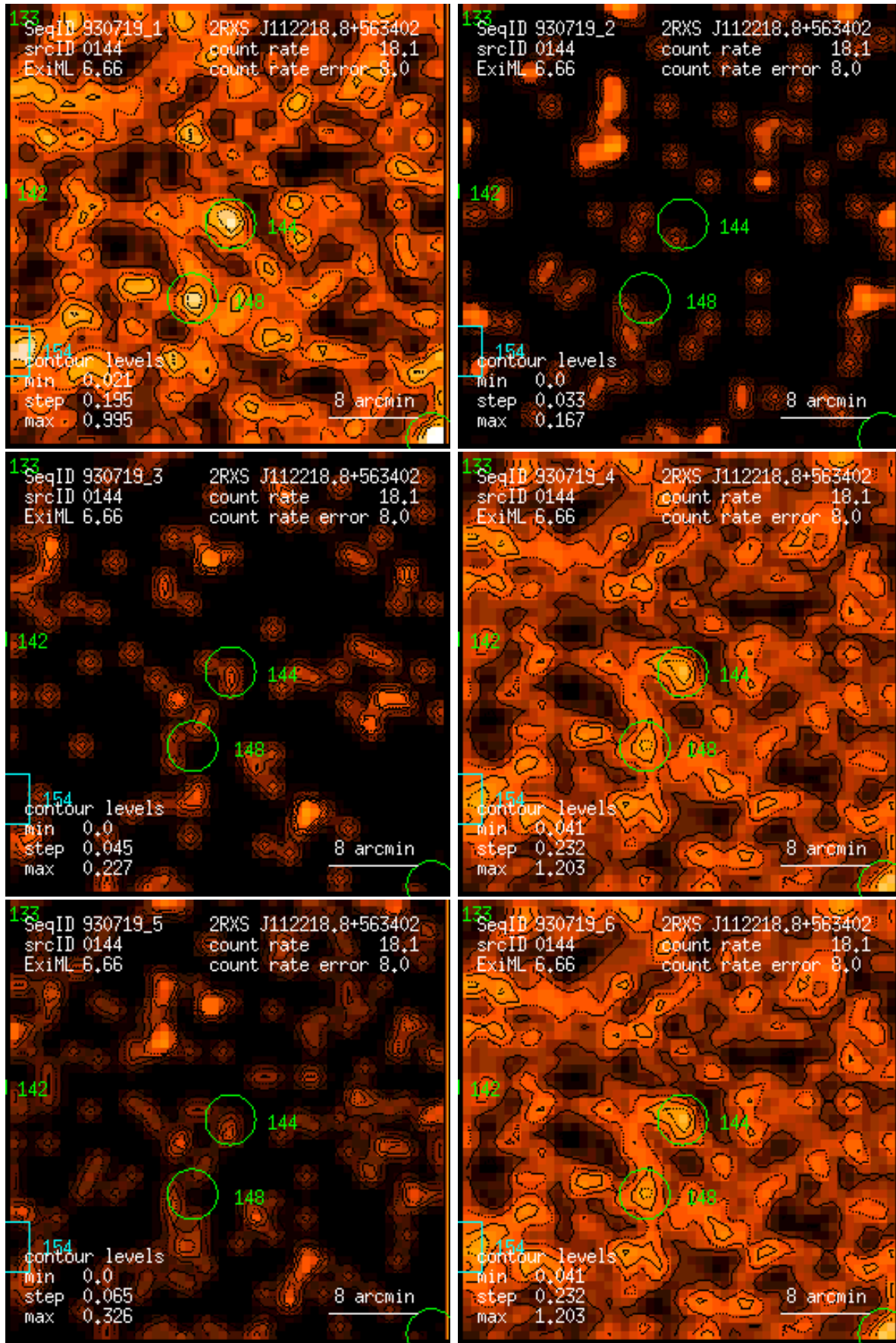
Figure 144: RASS 930719: detection 0144: band rate images, Gaussian filter: (1) PSPC channels 11 – 41, (2) 52 – 90, (3) 91 – 201, (4) 11 – 235, (5) 52 – 201, (6) 11 – 201. Broad band rates in counts/ks. Band rate contour levels in counts/ks/arcmin 2 .
