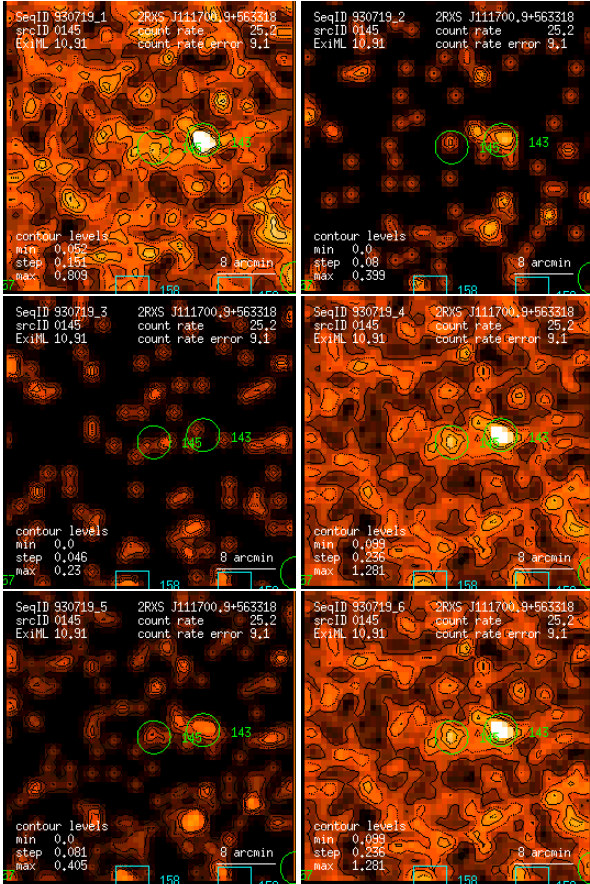
Figure 145: RASS 930719: detection 0145: band rate images, Gaussian filter: (1) PSPC channels 11 – 41, (2) 52 – 90, (3) 91 – 201, (4) 11 – 235, (5) 52 – 201, (6) 11 – 201. Broad band rates in counts/ks. Band rate contour levels in counts/ks/arcmin 2 .
