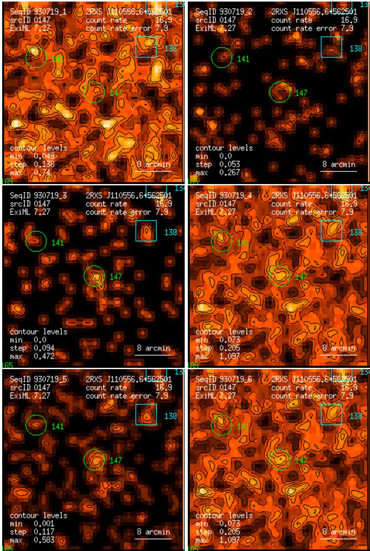
Figure 147: RASS 930719: detection 0147: band rate images, Gaussian filter: (1) PSPC channels 11 – 41, (2) 52 – 90, (3) 91 – 201, (4) 11 – 235, (5) 52 – 201, (6) 11 – 201. Broad band rates in counts/ks. Band rate contour levels in counts/ks/arcmin 2 .
