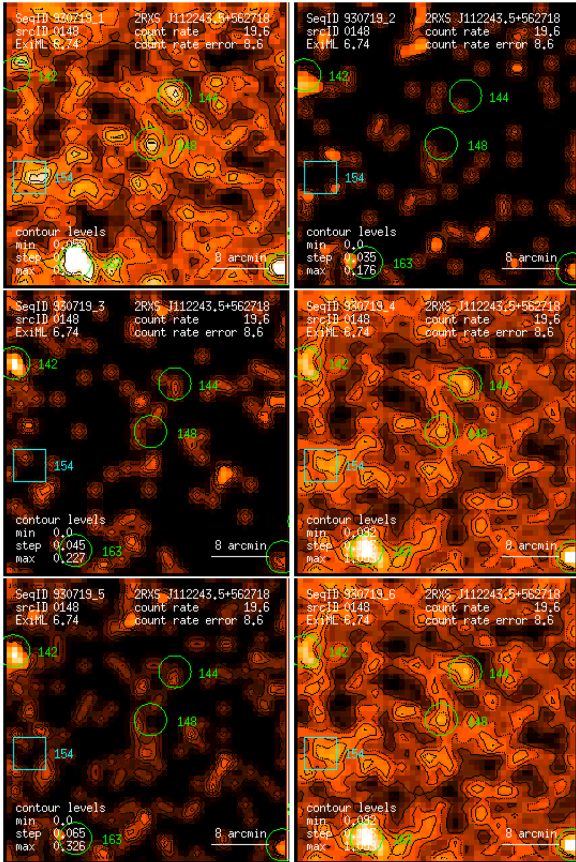
Figure 148: RASS 930719: detection 0148: band rate images, Gaussian filter: (1) PSPC channels 11 – 41, (2) 52 – 90, (3) 91 – 201, (4) 11 – 235, (5) 52 – 201, (6) 11 – 201. Broad band rates in counts/ks. Band rate contour levels in counts/ks/arcmin 2 .
