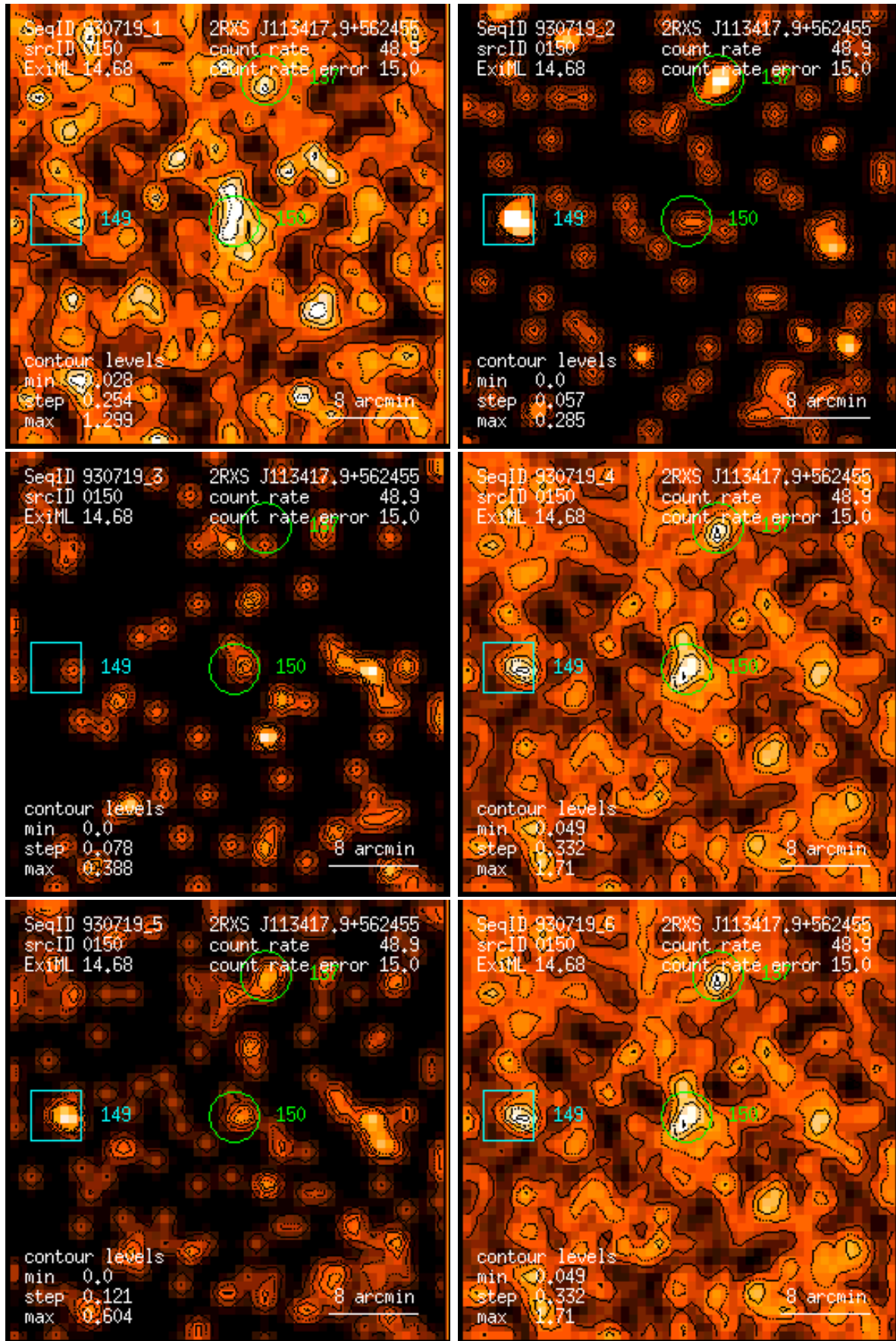
Figure 150: RASS 930719: detection 0150: band rate images, Gaussian filter: (1) PSPC channels 11 – 41, (2) 52 – 90, (3) 91 – 201, (4) 11 – 235, (5) 52 – 201, (6) 11 – 201. Broad band rates in counts/ks. Band rate contour levels in counts/ks/arcmin 2 .
