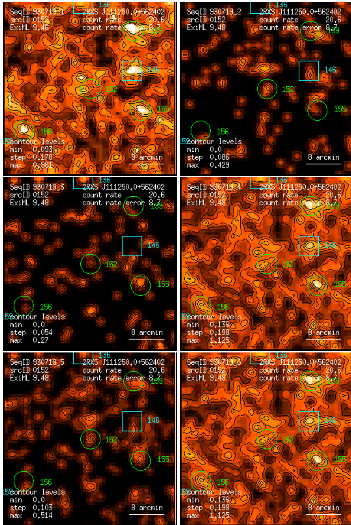
Figure 152: RASS 930719: detection 0152: band rate images, Gaussian filter: (1) PSPC channels 11 – 41, (2) 52 – 90, (3) 91 – 201, (4) 11 – 235, (5) 52 – 201, (6) 11 – 201. Broad band rates in counts/ks. Band rate contour levels in counts/ks/arcmin 2 .
