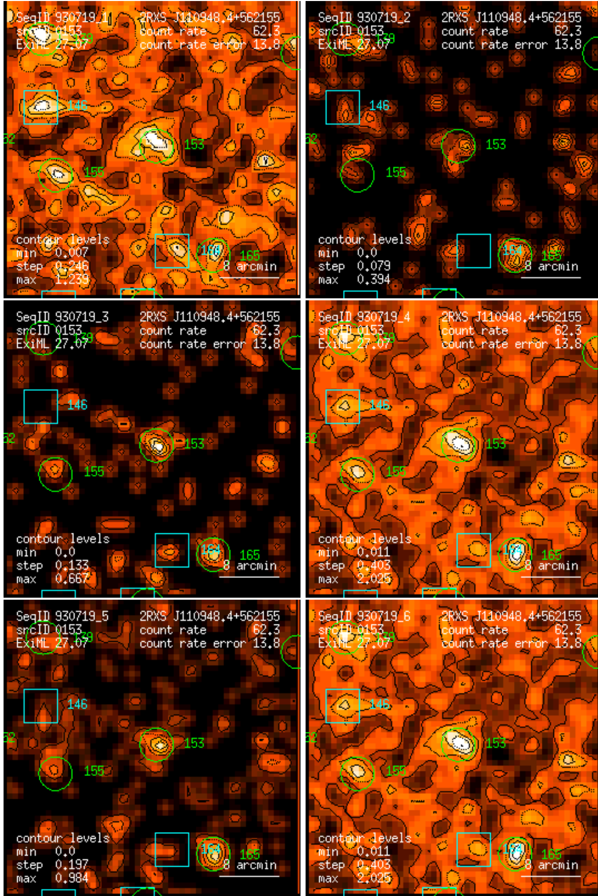
Figure 153: RASS 930719: detection 0153: band rate images, Gaussian filter: (1) PSPC channels 11 – 41, (2) 52 – 90, (3) 91 – 201, (4) 11 – 235, (5) 52 – 201, (6) 11 – 201. Broad band rates in counts/ks. Band rate contour levels in counts/ks/arcmin 2 .
