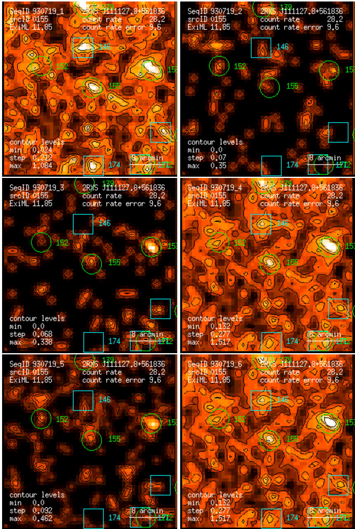
Figure 155: RASS 930719: detection 0155: band rate images, Gaussian filter: (1) PSPC channels 11 – 41, (2) 52 – 90, (3) 91 – 201, (4) 11 – 235, (5) 52 – 201, (6) 11 – 201. Broad band rates in counts/ks. Band rate contour levels in counts/ks/arcmin 2 .
