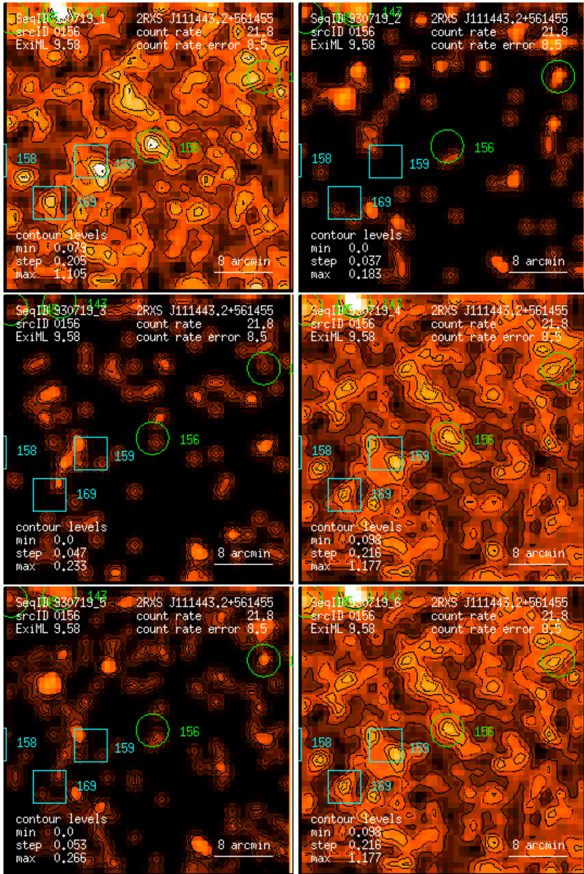
Figure 156: RASS 930719: detection 0156: band rate images, Gaussian filter: (1) PSPC channels 11 – 41, (2) 52 – 90, (3) 91 – 201, (4) 11 – 235, (5) 52 – 201, (6) 11 – 201. Broad band rates in counts/ks. Band rate contour levels in counts/ks/arcmin 2 .
