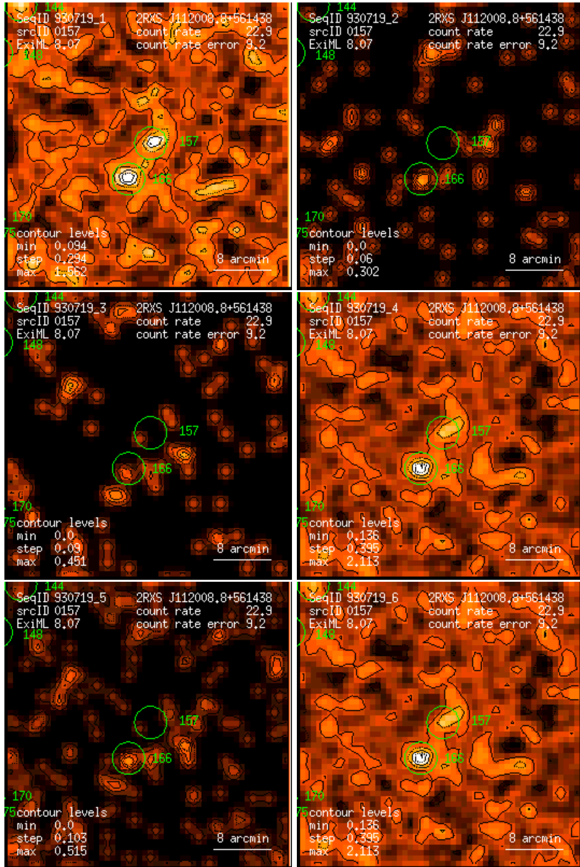
Figure 157: RASS 930719: detection 0157: band rate images, Gaussian filter: (1) PSPC channels 11 – 41, (2) 52 – 90, (3) 91 – 201, (4) 11 – 235, (5) 52 – 201, (6) 11 – 201. Broad band rates in counts/ks. Band rate contour levels in counts/ks/arcmin 2 .
