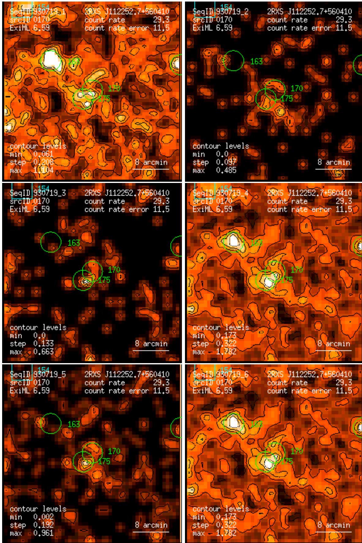
Figure 170: RASS 930719: detection 0170: band rate images, Gaussian filter: (1) PSPC channels 11 – 41, (2) 52 – 90, (3) 91 – 201, (4) 11 – 235, (5) 52 – 201, (6) 11 – 201. Broad band rates in counts/ks. Band rate contour levels in counts/ks/arcmin 2 .
