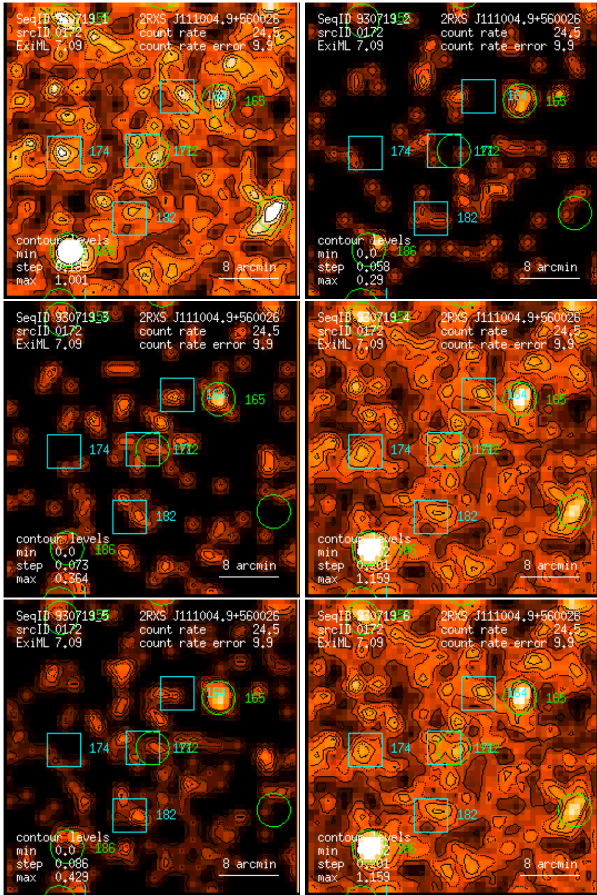
Figure 172: RASS 930719: detection 0172: band rate images, Gaussian filter: (1) PSPC channels 11 – 41, (2) 52 – 90, (3) 91 – 201, (4) 11 – 235, (5) 52 – 201, (6) 11 – 201. Broad band rates in counts/ks. Band rate contour levels in counts/ks/arcmin 2 .
