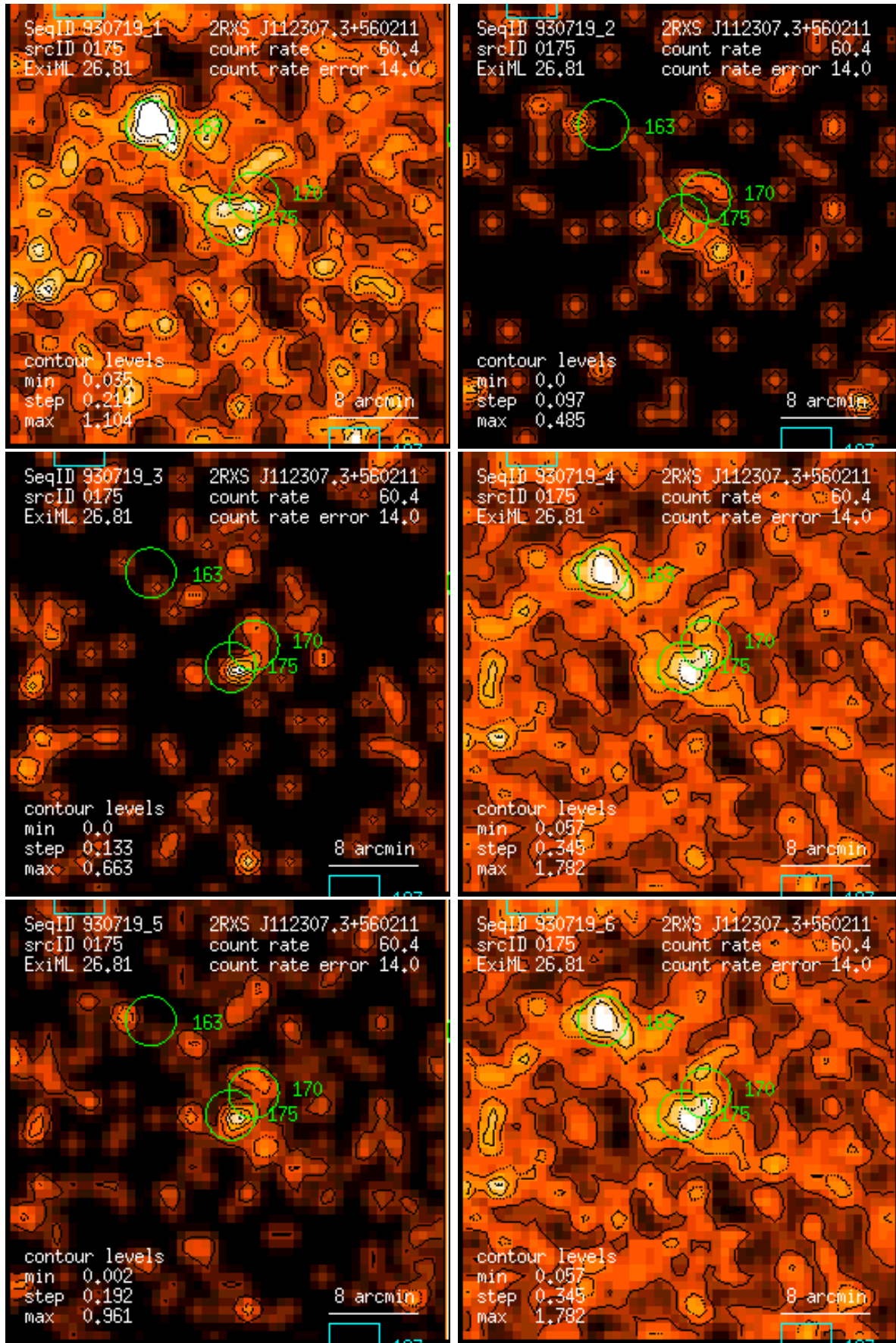
Figure 175: RASS 930719: detection 0175: band rate images, Gaussian filter: (1) PSPC channels 11 – 41, (2) 52 – 90, (3) 91 – 201, (4) 11 – 235, (5) 52 – 201, (6) 11 – 201. Broad band rates in counts/ks. Band rate contour levels in counts/ks/arcmin 2 .
