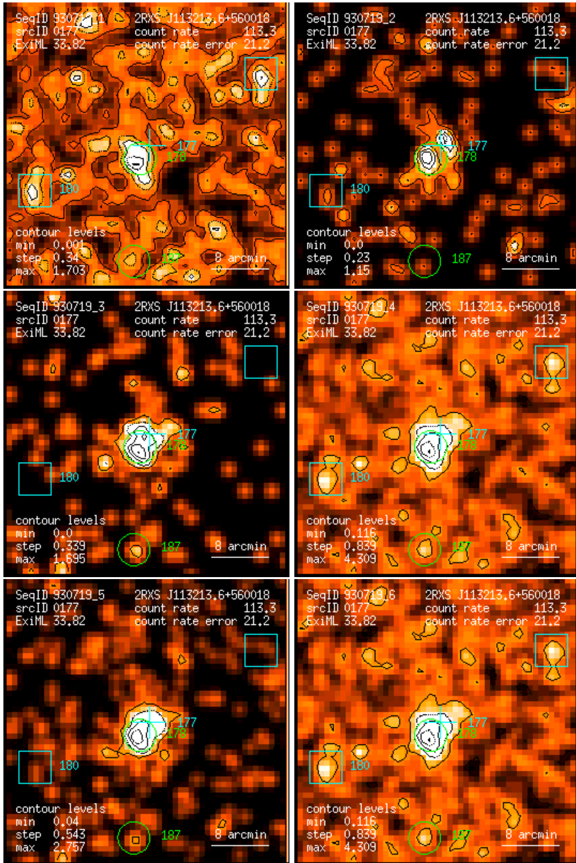
Figure 177: RASS 930719: detection 0177: band rate images, Gaussian filter: (1) PSPC channels 11 – 41, (2) 52 – 90, (3) 91 – 201, (4) 11 – 235, (5) 52 – 201, (6) 11 – 201. Broad band rates in counts/ks. Band rate contour levels in counts/ks/arcmin 2 .
