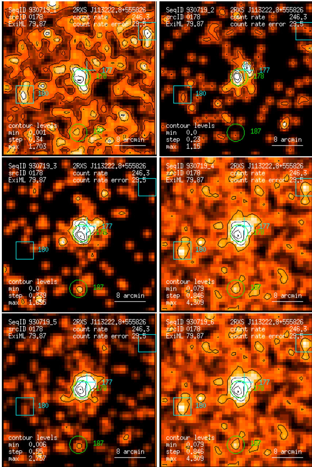
Figure 178: RASS 930719: detection 0178: band rate images, Gaussian filter: (1) PSPC channels 11 – 41, (2) 52 – 90, (3) 91 – 201, (4) 11 – 235, (5) 52 – 201, (6) 11 – 201. Broad band rates in counts/ks. Band rate contour levels in counts/ks/arcmin 2 .
