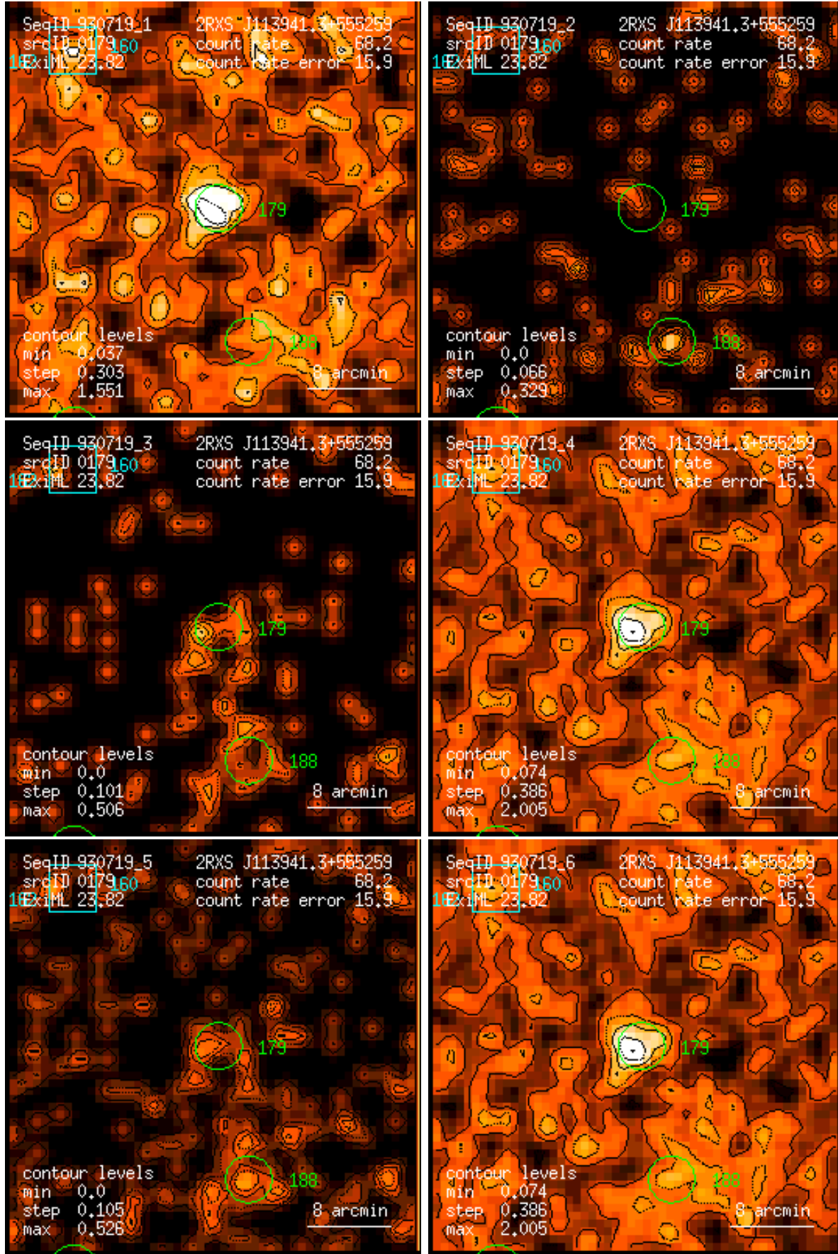
Figure 179: RASS 930719: detection 0179: band rate images, Gaussian filter: (1) PSPC channels 11 – 41, (2) 52 – 90, (3) 91 – 201, (4) 11 – 235, (5) 52 – 201, (6) 11 – 201. Broad band rates in counts/ks. Band rate contour levels in counts/ks/arcmin 2 .
