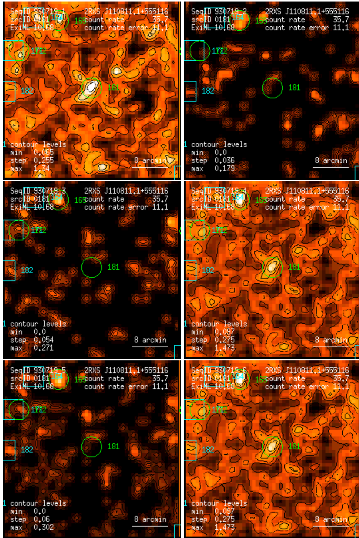
Figure 181: RASS 930719: detection 0181: band rate images, Gaussian filter: (1) PSPC channels 11 – 41, (2) 52 – 90, (3) 91 – 201, (4) 11 – 235, (5) 52 – 201, (6) 11 – 201. Broad band rates in counts/ks. Band rate contour levels in counts/ks/arcmin 2 .
