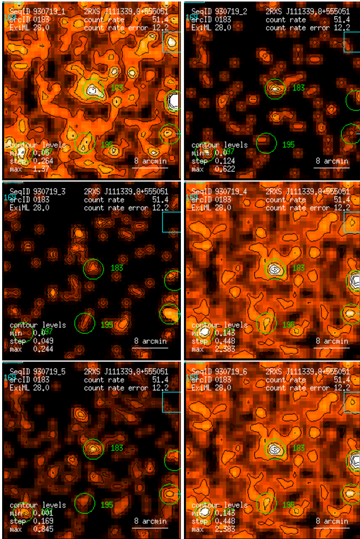
Figure 183: RASS 930719: detection 0183: band rate images, Gaussian filter: (1) PSPC channels 11 – 41, (2) 52 – 90, (3) 91 – 201, (4) 11 – 235, (5) 52 – 201, (6) 11 – 201. Broad band rates in counts/ks. Band rate contour levels in counts/ks/arcmin 2 .
