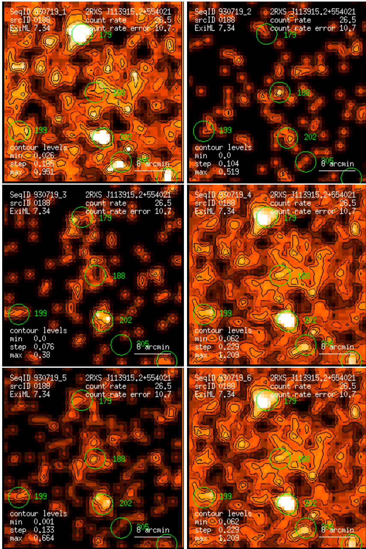
Figure 188: RASS 930719: detection 0188: band rate images, Gaussian filter: (1) PSPC channels 11 – 41, (2) 52 – 90, (3) 91 – 201, (4) 11 – 235, (5) 52 – 201, (6) 11 – 201. Broad band rates in counts/ks. Band rate contour levels in counts/ks/arcmin 2 .
