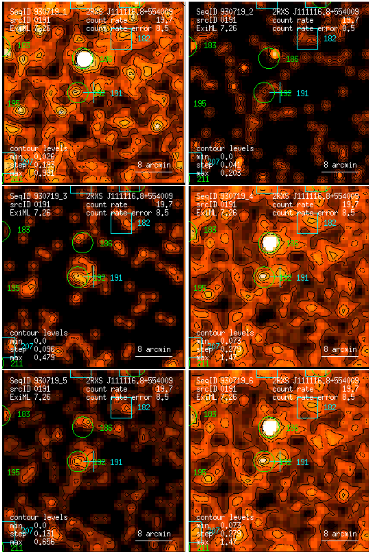
Figure 191: RASS 930719: detection 0191: band rate images, Gaussian filter: (1) PSPC channels 11 – 41, (2) 52 – 90, (3) 91 – 201, (4) 11 – 235, (5) 52 – 201, (6) 11 – 201. Broad band rates in counts/ks. Band rate contour levels in counts/ks/arcmin 2 .
