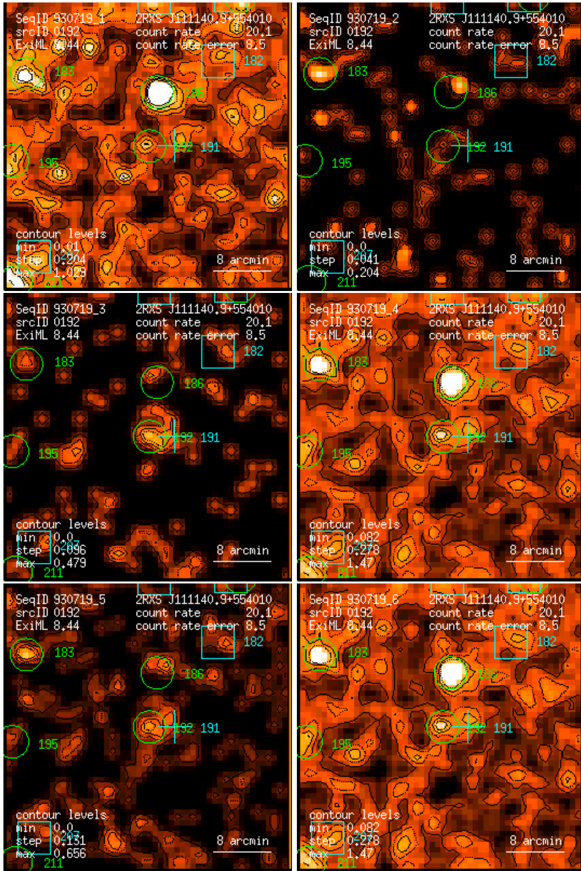
Figure 192: RASS 930719: detection 0192: band rate images, Gaussian filter: (1) PSPC channels 11 – 41, (2) 52 – 90, (3) 91 – 201, (4) 11 – 235, (5) 52 – 201, (6) 11 – 201. Broad band rates in counts/ks. Band rate contour levels in counts/ks/arcmin 2 .
