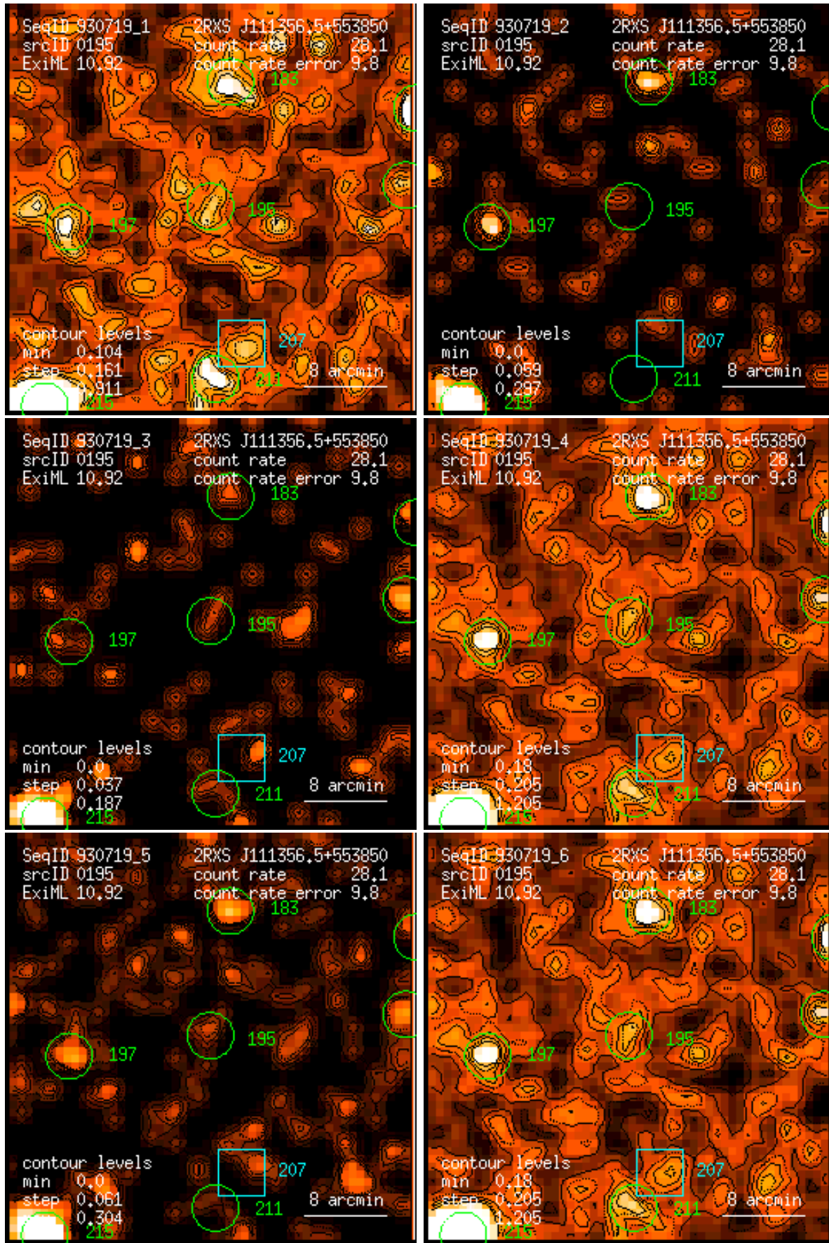
Figure 195: RASS 930719: detection 0195: band rate images, Gaussian filter: (1) PSPC channels 11 – 41, (2) 52 – 90, (3) 91 – 201, (4) 11 – 235, (5) 52 – 201, (6) 11 – 201. Broad band rates in counts/ks. Band rate contour levels in counts/ks/arcmin 2 .
