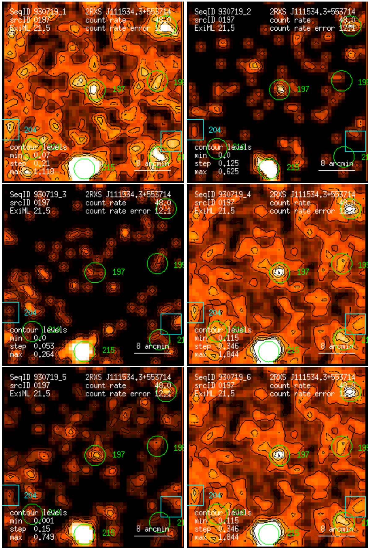
Figure 197: RASS 930719: detection 0197: band rate images, Gaussian filter: (1) PSPC channels 11 – 41, (2) 52 – 90, (3) 91 – 201, (4) 11 – 235, (5) 52 – 201, (6) 11 – 201. Broad band rates in counts/ks. Band rate contour levels in counts/ks/arcmin 2 .
