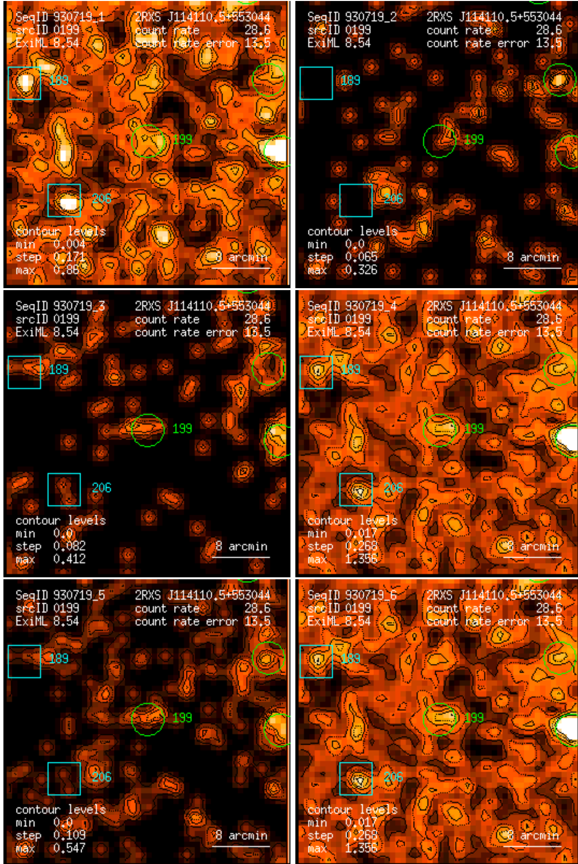
Figure 199: RASS 930719: detection 0199: band rate images, Gaussian filter: (1) PSPC channels 11 – 41, (2) 52 – 90, (3) 91 – 201, (4) 11 – 235, (5) 52 – 201, (6) 11 – 201. Broad band rates in counts/ks. Band rate contour levels in counts/ks/arcmin 2 .
