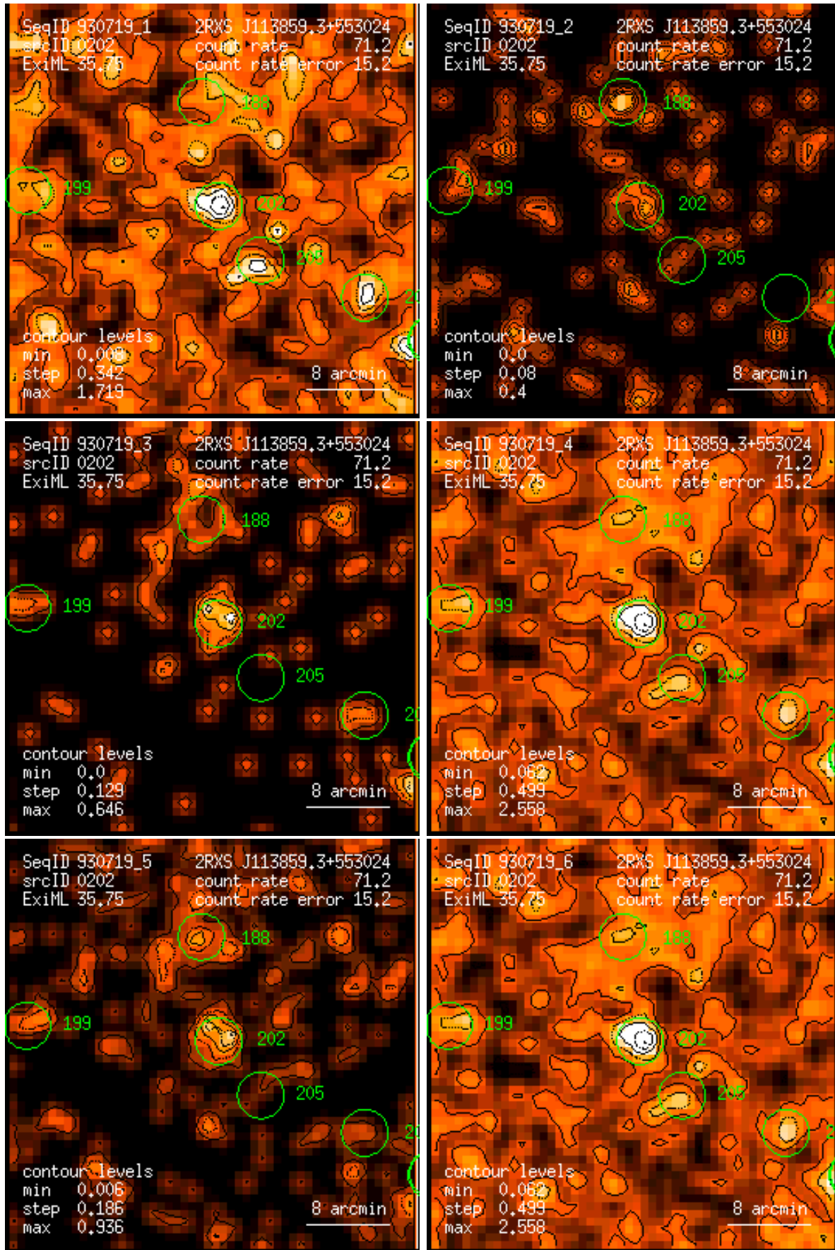
Figure 202: RASS 930719: detection 0202: band rate images, Gaussian filter: (1) PSPC channels 11 – 41, (2) 52 – 90, (3) 91 – 201, (4) 11 – 235, (5) 52 – 201, (6) 11 – 201. Broad band rates in counts/ks. Band rate contour levels in counts/ks/arcmin 2 .
