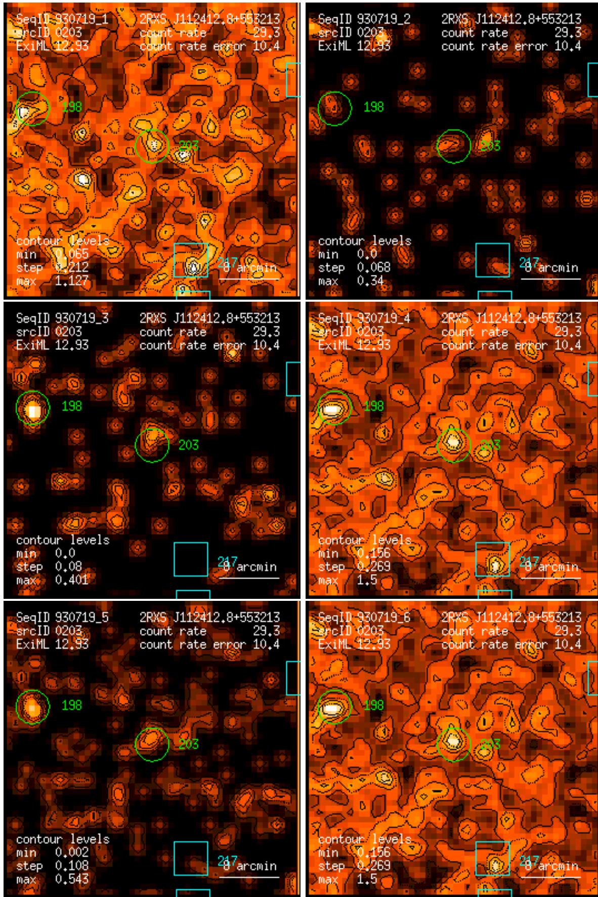
Figure 203: RASS 930719: detection 0203: band rate images, Gaussian filter: (1) PSPC channels 11 – 41, (2) 52 – 90, (3) 91 – 201, (4) 11 – 235, (5) 52 – 201, (6) 11 – 201. Broad band rates in counts/ks. Band rate contour levels in counts/ks/arcmin 2 .
