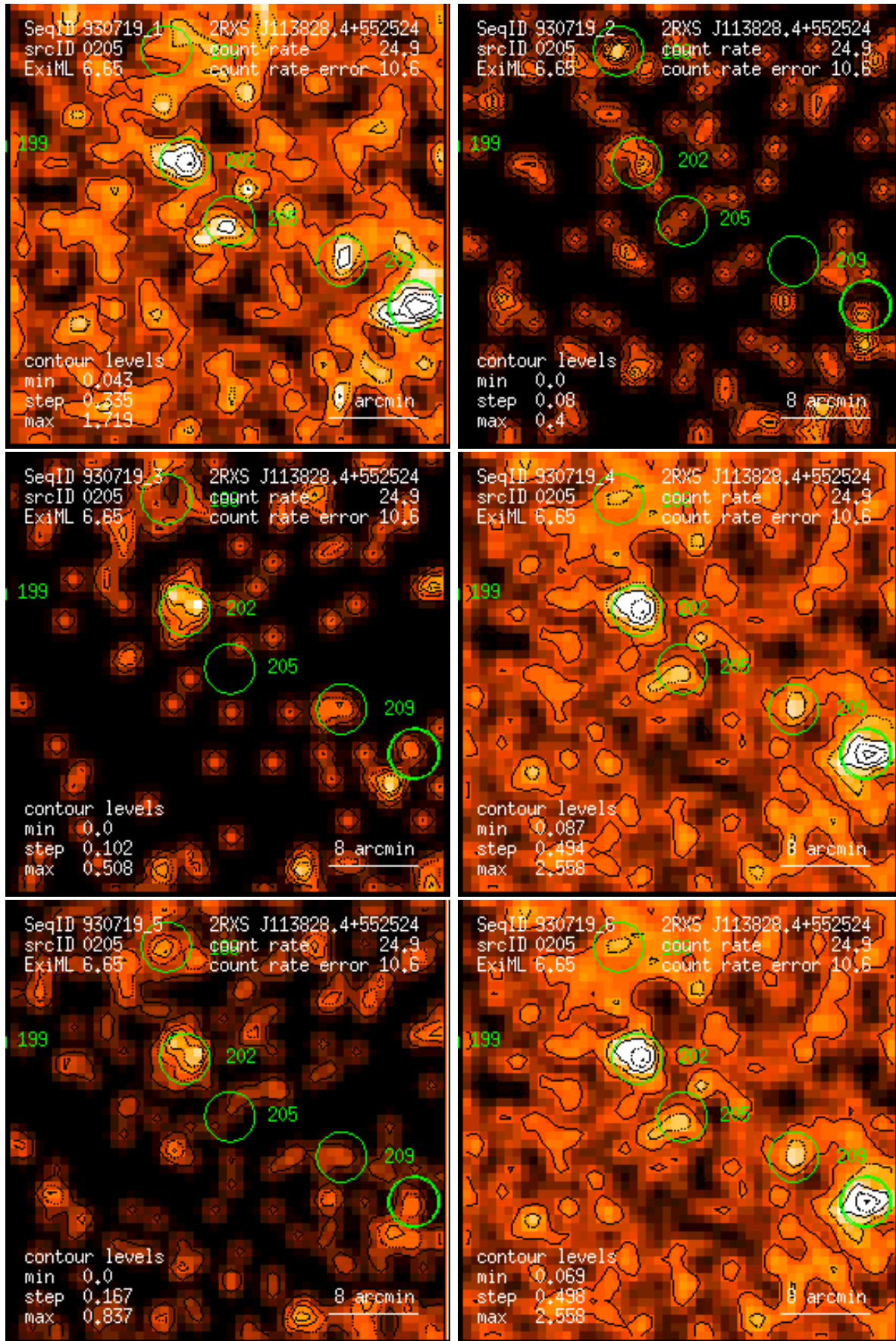
Figure 205: RASS 930719: detection 0205: band rate images, Gaussian filter: (1) PSPC channels 11 – 41, (2) 52 – 90, (3) 91 – 201, (4) 11 – 235, (5) 52 – 201, (6) 11 – 201. Broad band rates in counts/ks. Band rate contour levels in counts/ks/arcmin 2 .
