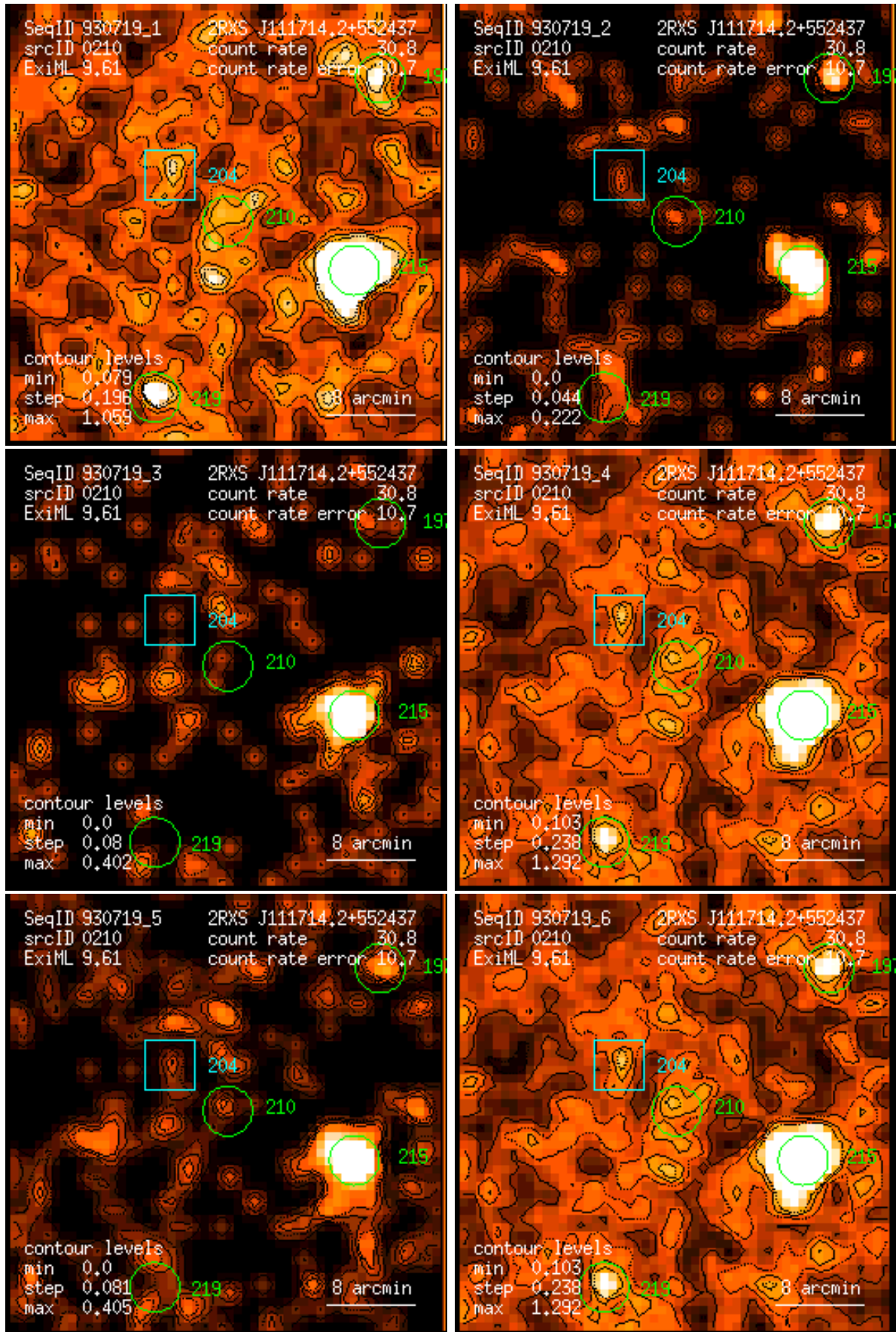
Figure 210: RASS 930719: detection 0210: band rate images, Gaussian filter: (1) PSPC channels 11 – 41, (2) 52 – 90, (3) 91 – 201, (4) 11 – 235, (5) 52 – 201, (6) 11 – 201. Broad band rates in counts/ks. Band rate contour levels in counts/ks/arcmin 2 .
