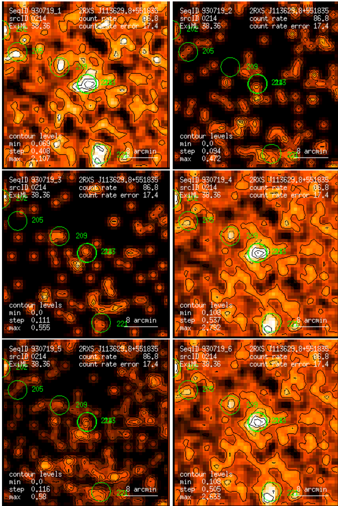
Figure 214: RASS 930719: detection 0214: band rate images, Gaussian filter: (1) PSPC channels 11 – 41, (2) 52 – 90, (3) 91 – 201, (4) 11 – 235, (5) 52 – 201, (6) 11 – 201. Broad band rates in counts/ks. Band rate contour levels in counts/ks/arcmin 2 .
