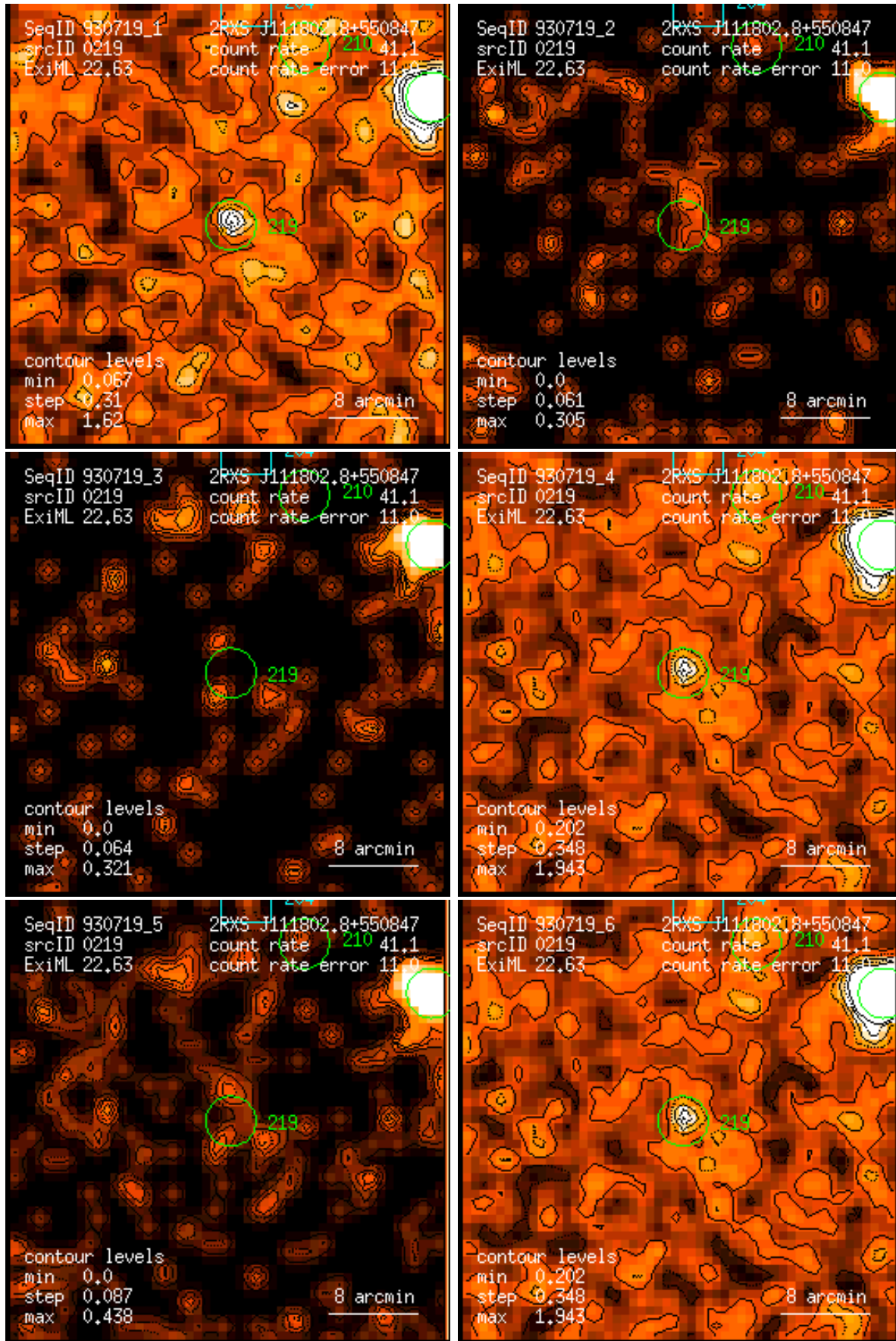
Figure 219: RASS 930719: detection 0219: band rate images, Gaussian filter: (1) PSPC channels 11 – 41, (2) 52 – 90, (3) 91 – 201, (4) 11 – 235, (5) 52 – 201, (6) 11 – 201. Broad band rates in counts/ks. Band rate contour levels in counts/ks/arcmin 2 .
