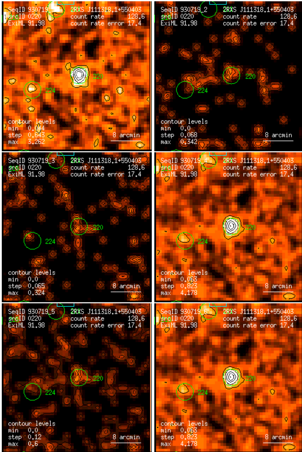
Figure 220: RASS 930719: detection 0220: band rate images, Gaussian filter: (1) PSPC channels 11 – 41, (2) 52 – 90, (3) 91 – 201, (4) 11 – 235, (5) 52 – 201, (6) 11 – 201. Broad band rates in counts/ks. Band rate contour levels in counts/ks/arcmin 2 .
