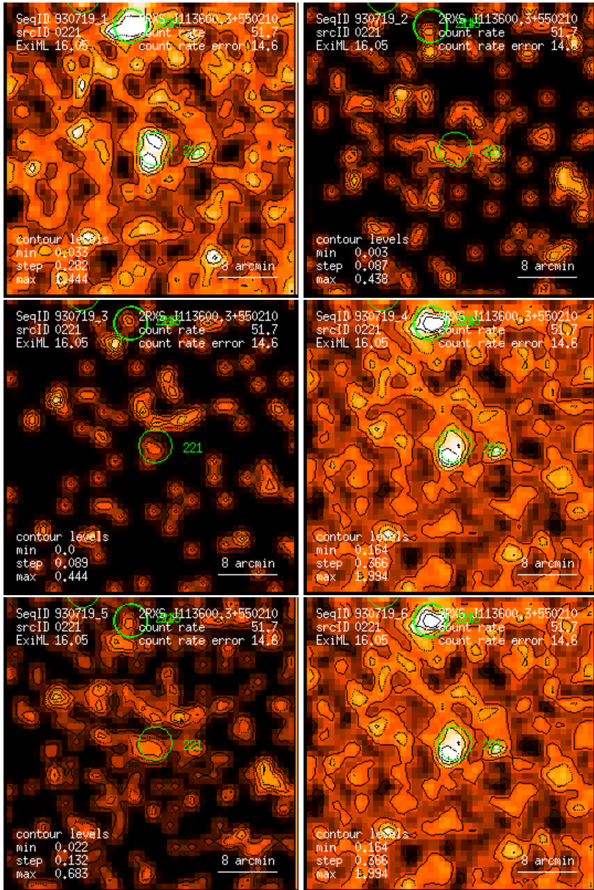
Figure 221: RASS 930719: detection 0221: band rate images, Gaussian filter: (1) PSPC channels 11 – 41, (2) 52 – 90, (3) 91 – 201, (4) 11 – 235, (5) 52 – 201, (6) 11 – 201. Broad band rates in counts/ks. Band rate contour levels in counts/ks/arcmin 2 .
