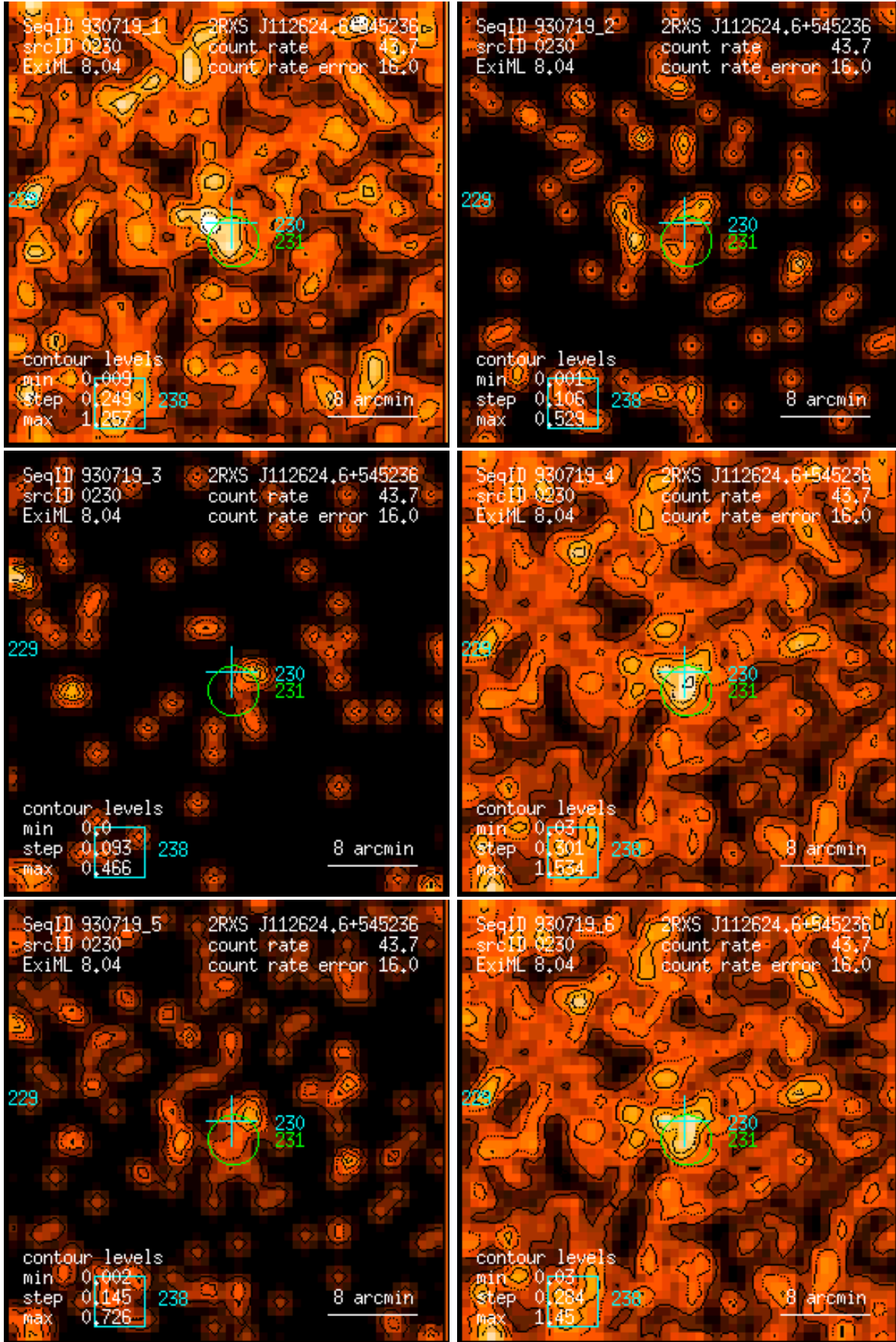
Figure 230: RASS 930719: detection 0230: band rate images, Gaussian filter: (1) PSPC channels 11 – 41, (2) 52 – 90, (3) 91 – 201, (4) 11 – 235, (5) 52 – 201, (6) 11 – 201. Broad band rates in counts/ks. Band rate contour levels in counts/ks/arcmin 2 .
