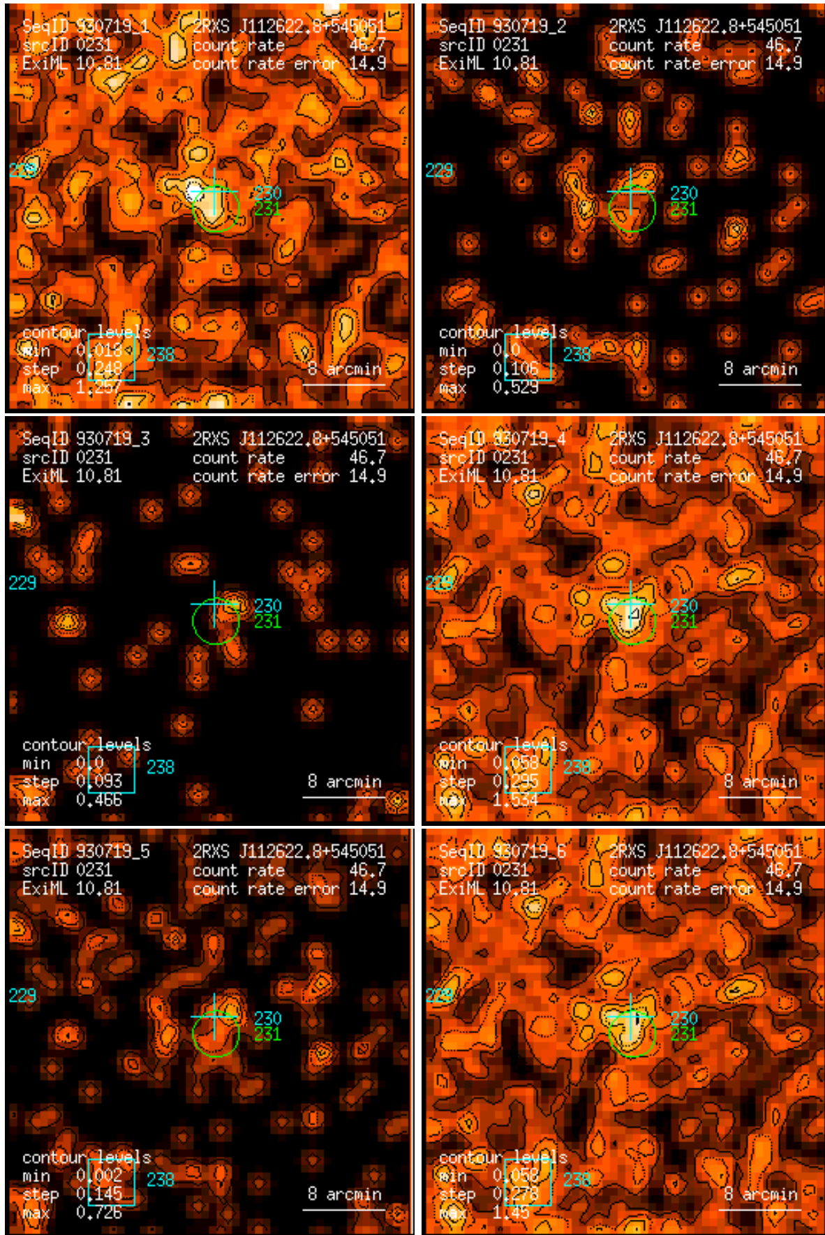
Figure 231: RASS 930719: detection 0231: band rate images, Gaussian filter: (1) PSPC channels 11 – 41, (2) 52 – 90, (3) 91 – 201, (4) 11 – 235, (5) 52 – 201, (6) 11 – 201. Broad band rates in counts/ks. Band rate contour levels in counts/ks/arcmin 2 .
