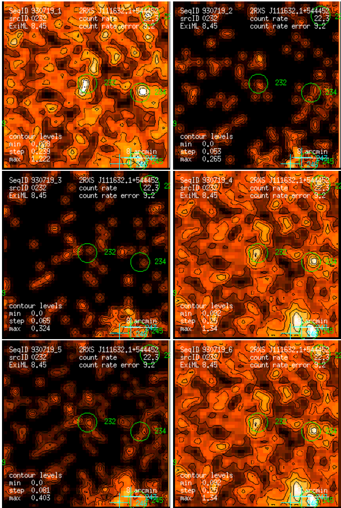
Figure 232: RASS 930719: detection 0232: band rate images, Gaussian filter: (1) PSPC channels 11 – 41, (2) 52 – 90, (3) 91 – 201, (4) 11 – 235, (5) 52 – 201, (6) 11 – 201. Broad band rates in counts/ks. Band rate contour levels in counts/ks/arcmin 2 .
